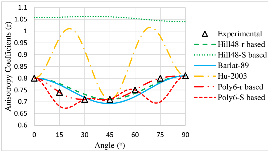
Fig. 6 Angular variation of anisotropy coefficients for AA5XXX alloy
