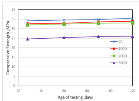
Fig. 10 Compressive strength results of quarry dust series
