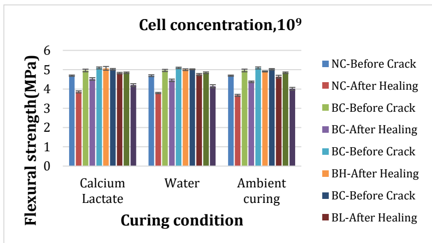
Fig. 6 Flexural strength of bacteria cell concentration of 10^9
