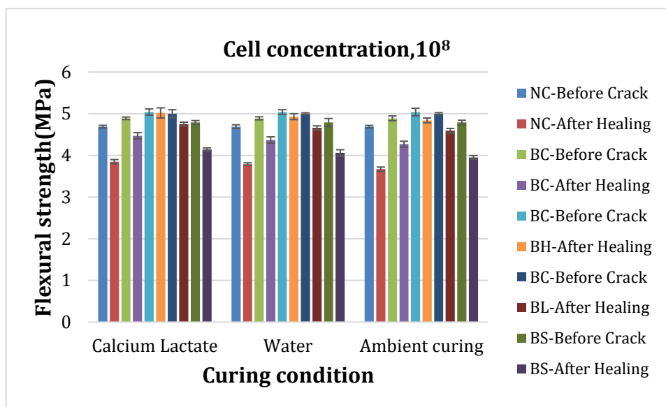
Fig. 7 Flexural strength of bacteria cell concentration of 10^8
