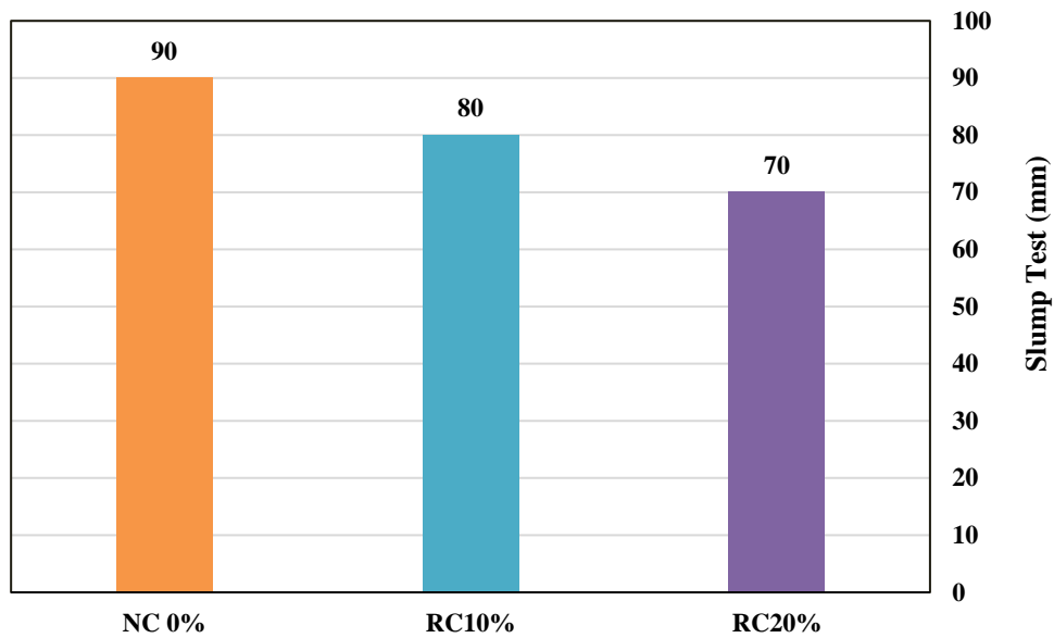
Fig. 4. The results of the slump test for both regular and rubberized concrete mixtures with varying rubber contents
