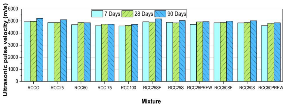
Fig. 11. Progression of UPV with time for RCC mixes
