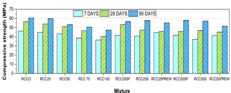
Fig. 9. Compressive strength of Roller-Compacted Concrete (RCC) at various substitution rates
