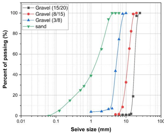
Fig. 3. Particle size distribution curves of the RCA used
