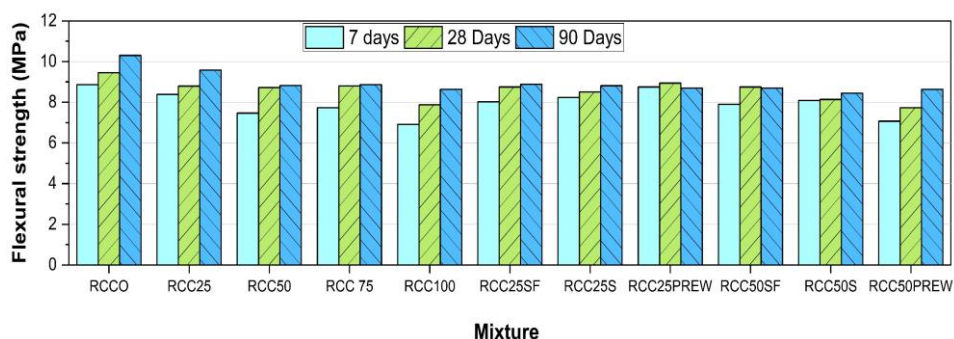
Fig. 10. Flexural strength of Roller-Compacted Concrete (RCC) at various substitution rates
