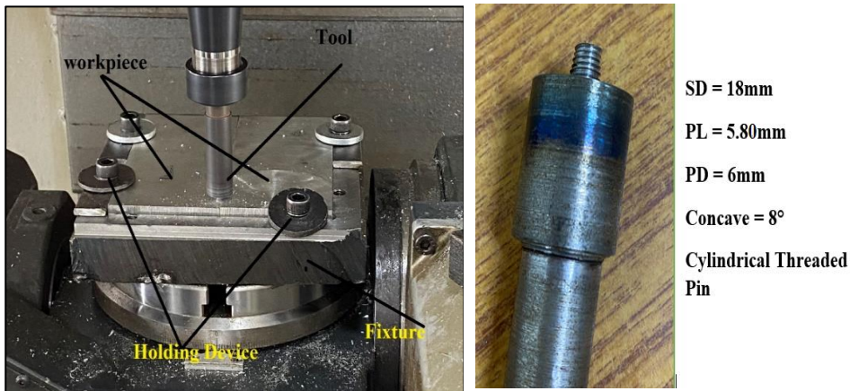
Fig. 2. Fixture and tool used in the FS-welding process
