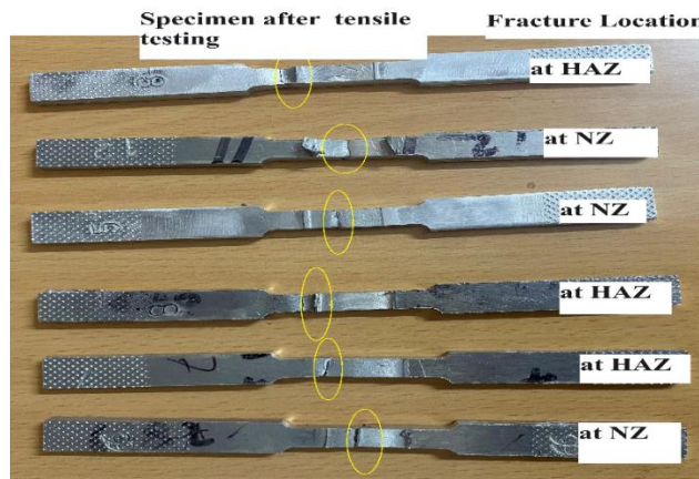
Fig. 16. Tensile specimens of welding aluminium alloys and failure locations
