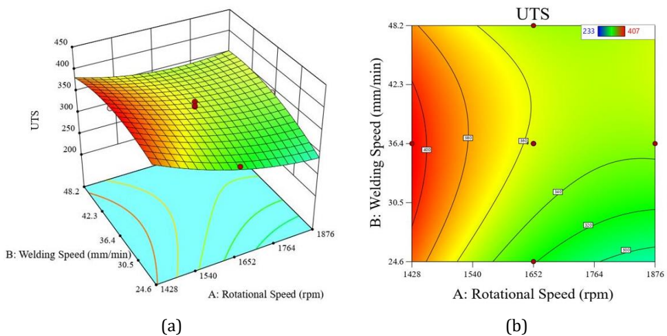
Fig.e 10. (a) Three-dimensional response and (b) contour plot for UTS
