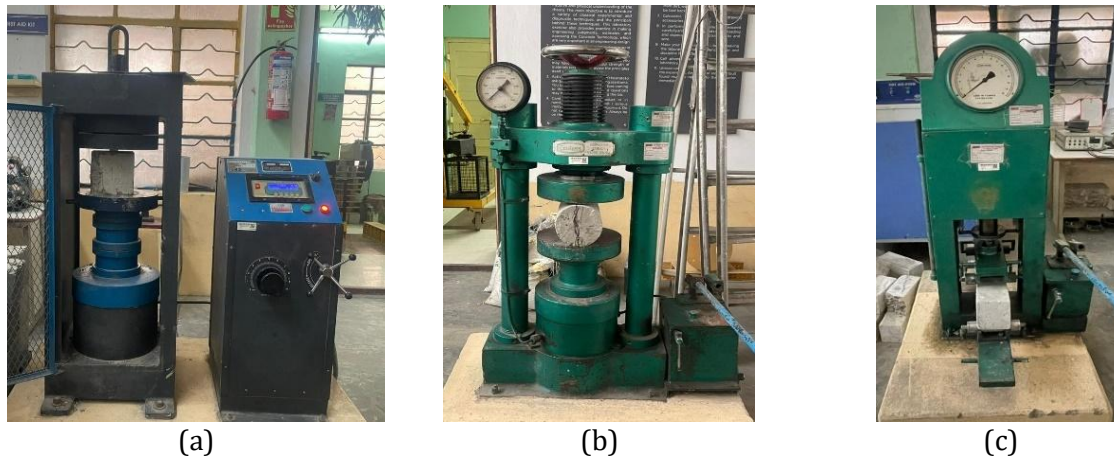
Fig. 7. Experimental setup (a) compression strength test, (b) split tensile test &amp; (c) flexural strength test
