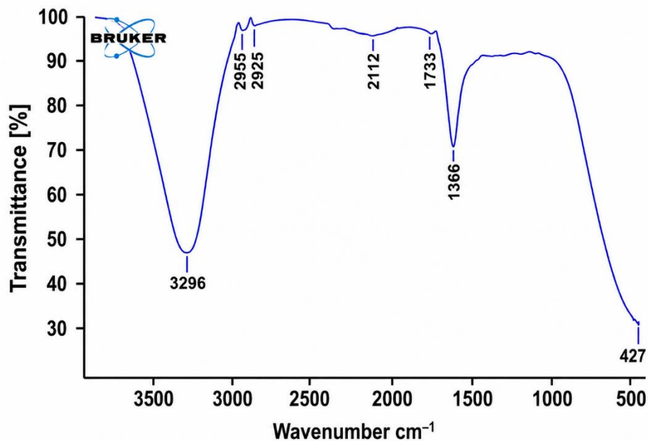
Fig. 10. Effect of ultrasound on oil sample by FTIR device
