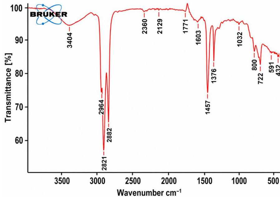
Fig. 11. FTIR examination of an oil sample before exposure to ultrasound
