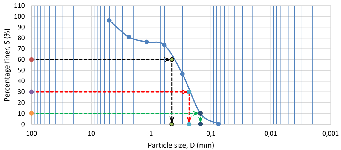
Fig. 13. Grading curve of RCA
