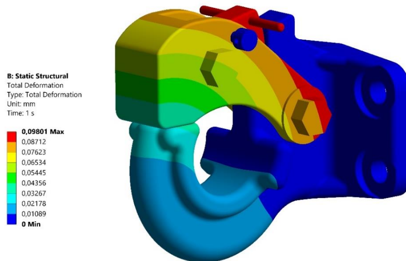
Fig. 11. Total deformation
