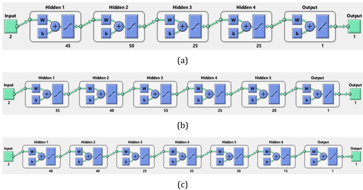
Fig. 11. The design of the NN with (a) four hidden layers, (b) five hidden layers, and (c) six hidden layers
