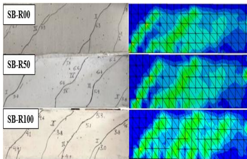
Fig. 9. Comparative crack pattern of solid beams
