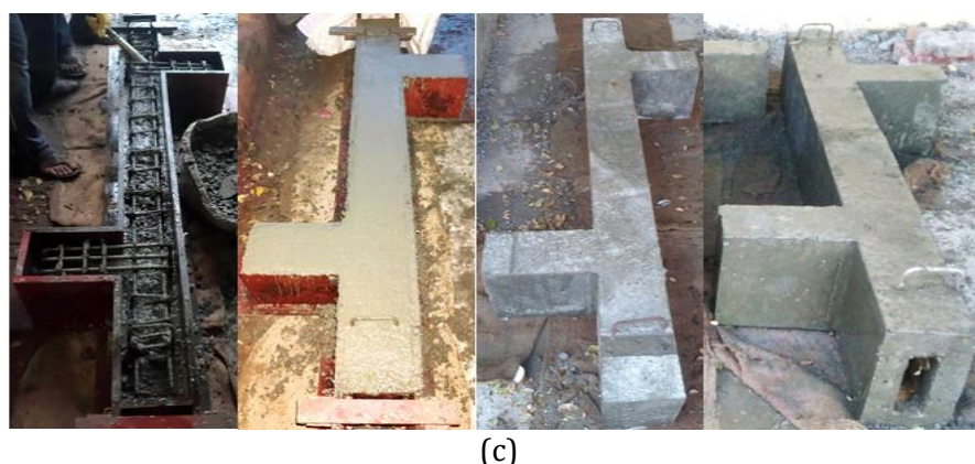
Fig. 4. Casting of beams
