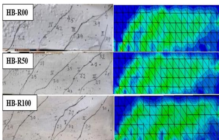
Fig. 10. Comparative crack pattern of Hollow beams
