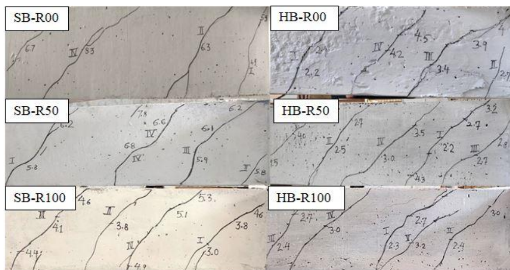
Fig. 6. Cracks pattern in test region of solid and hollow beams
