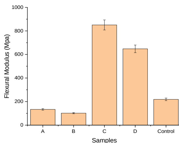
Fig. 11. Flexural modulus of BF/RH/ES reinforced polymer matrix composite
