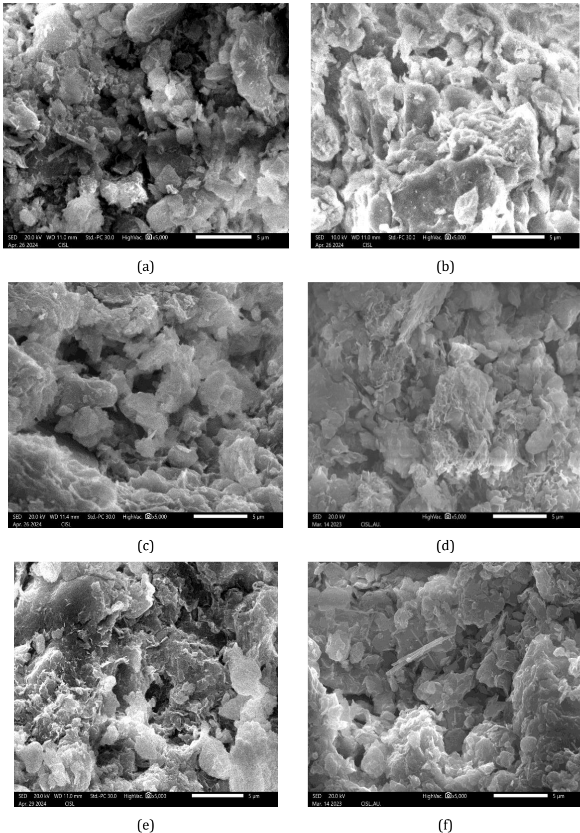
Fig. 7. Microstructural images (SEM) of soil samples stabilized with lime + copper slag (a) Soil + 8% lime with 2% slag, (b) Soil + 8% lime with 4% slag, (c) Soil + 8% lime with 6% slag, (d) Soil + 8% lime with 8% slag, (e) Soil + 8% lime with 10% slag and (f) Soil + 8% lime with 12% slag
