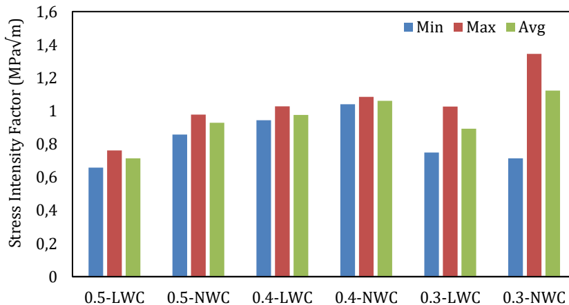
Fig. 17. Stress intensity factor
