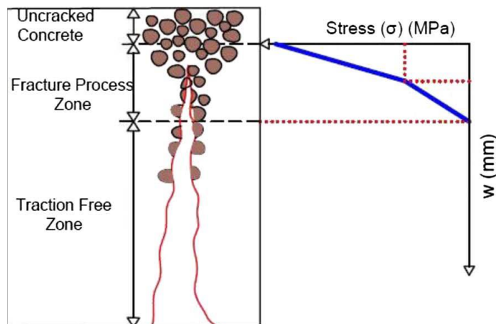
Fig. 1. Stress-crack width response of structural lightweight aggregate concrete [14]
