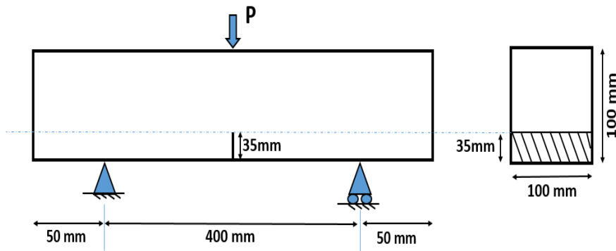
Fig. 7. Three-point bend test diagram
