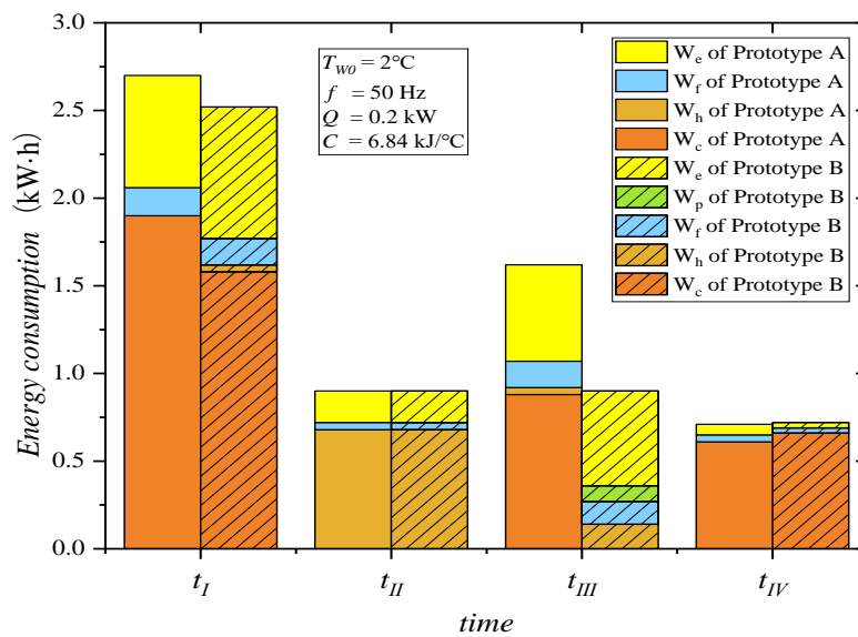
Fig. 12. Energy consumption distribution with Q = 0.2 \text{ kW}
