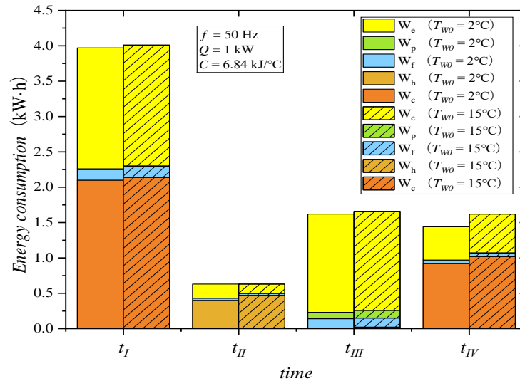
Fig. 14. Energy consumption distribution for Prototype B with T_{w0} = 15^\circ\text{C}
