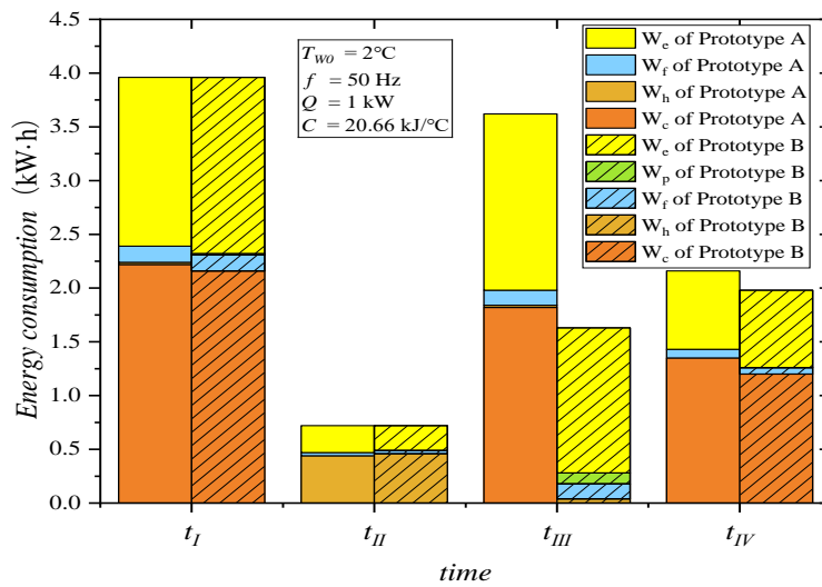
Fig. 10. Energy consumption distribution with C = 20.66 \text{ kJ/}^\circ\text{C}
