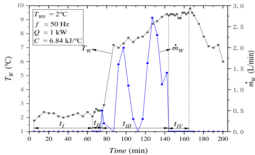
Fig. 7. Water temperature and flow rate of Prototype B under the nominal design conditions
