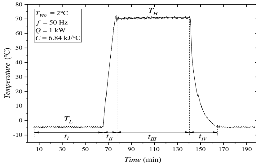
Fig. 5. Temperature curve of Prototype A under reference design conditions
