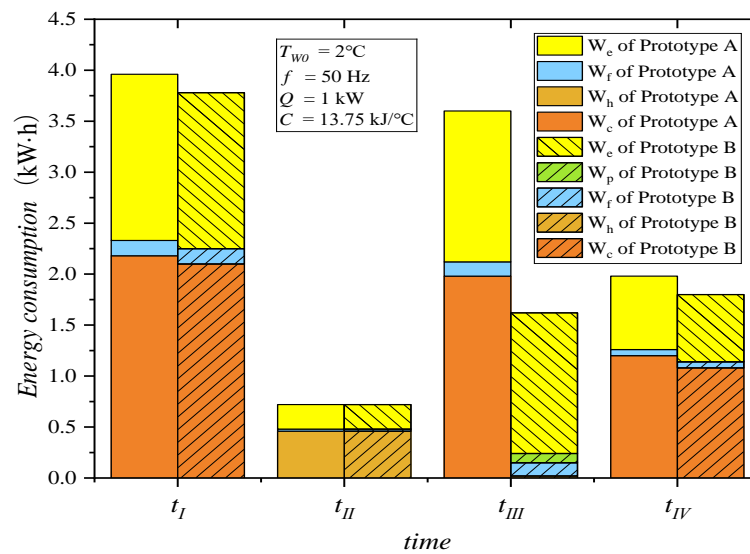
Fig. 9. Energy consumption distribution with C = 13.75 kJ/°C
