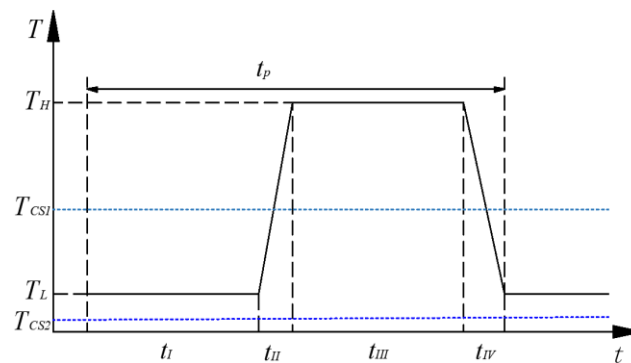
Fig. 15. The scheme of two cold storage temperatures
