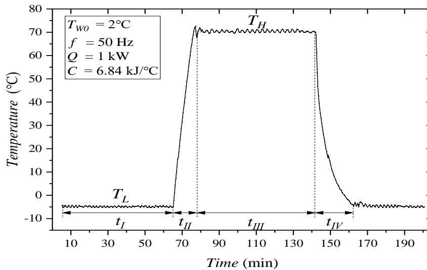
Fig. 6. Temperature curve of Prototype B under reference design conditions
