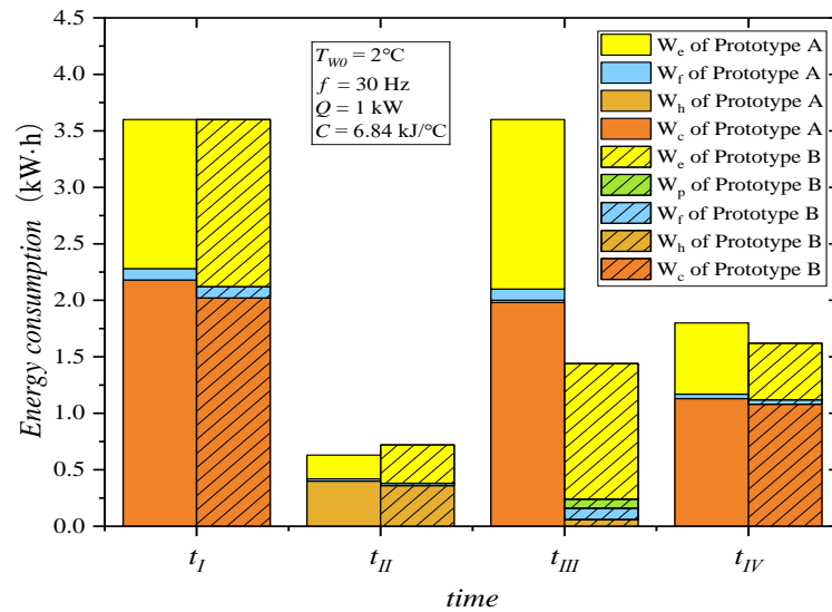
Fig. 13. Energy consumption distribution with f = 30 Hz
