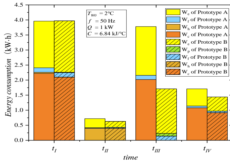
Fig. 8. Energy consumption distribution of Prototypes A and B under nominal design conditions
