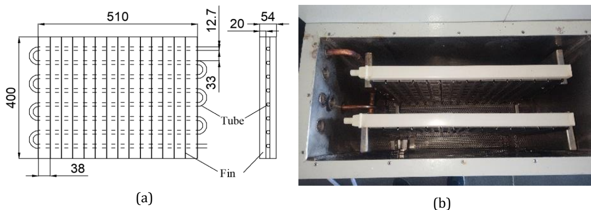
Fig. 3. Cold storage unit: (a) Dimensions (mm); (b) Photo of cold storage unit
