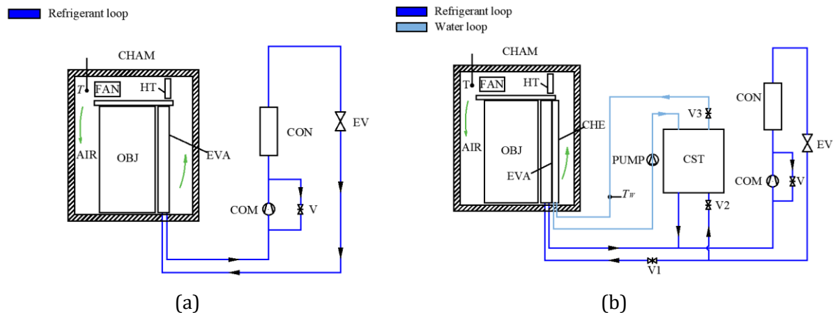
Fig. 2. Working principle: (a) prototype A; (b) prototype B
