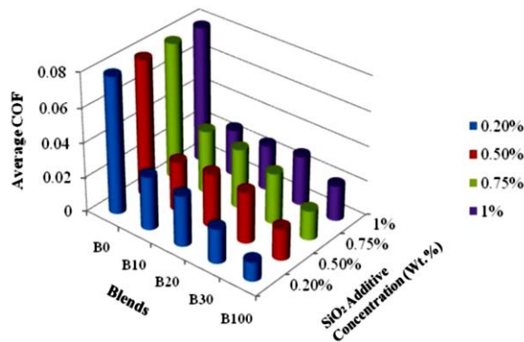
Fig. 23. General summing up of Change in Average COF for all permutations of SiO 2 nanoparticles
