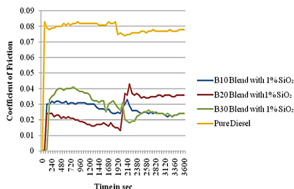
Fig. 12. Influence of 1% of \text{SiO}_2 nanoparticles in Laxmitaru-FAME in petro-diesel blends on COF
