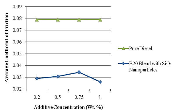
Fig. 16. Influence of % of \text{SiO}_2 nanoparticles in Simarouba glauca Methyl Ester for B20 blends on average friction
