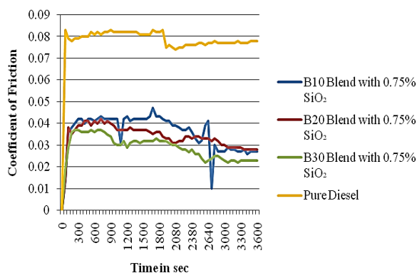
Fig. 11. Influence of 0.75% of \text{SiO}_2 nanoparticles in Laxmitaru-FAME in petro-diesel blends on COF
