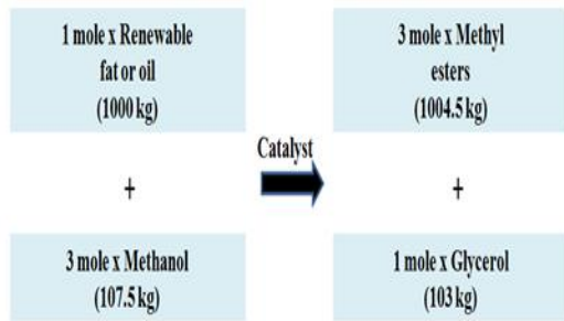
Fig. 1. Chemical reaction for biodiesel production [19]
