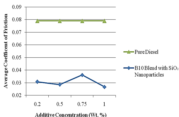
Fig. 15. Influence of % of \text{SiO}_2 nanoparticles in Simarouba glauca Methyl Ester for B10 blends on average friction
