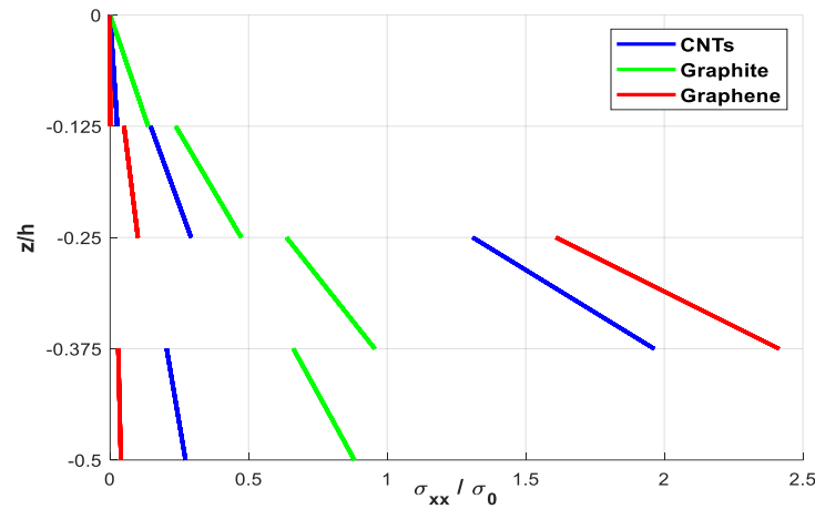
Fig. 3. Distribution of [45^\circ/0^\circ/-45^\circ/90^\circ]_s for dimensionless normal stress across normalized thickness
