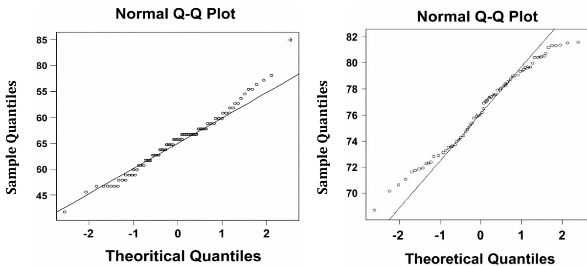
Fig. 3. Q-Q plot for noise level on the left and speed level on the right
