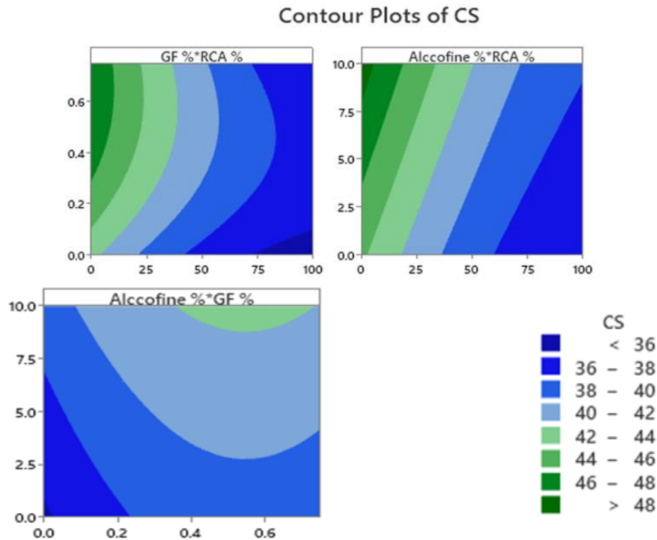
Fig. 17. Contour plots among the variables for CS
