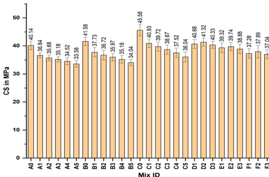
Fig. 5. Variations in Compressive strength outcomes after 28 days
