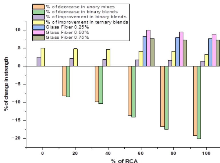
Fig. 11. Variation in modulus of elasticity
