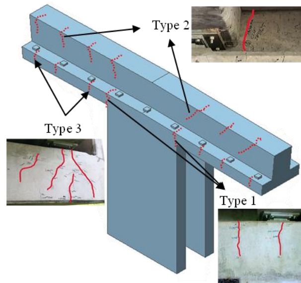
(b) Three-dimensional schematic view of crack patterns
