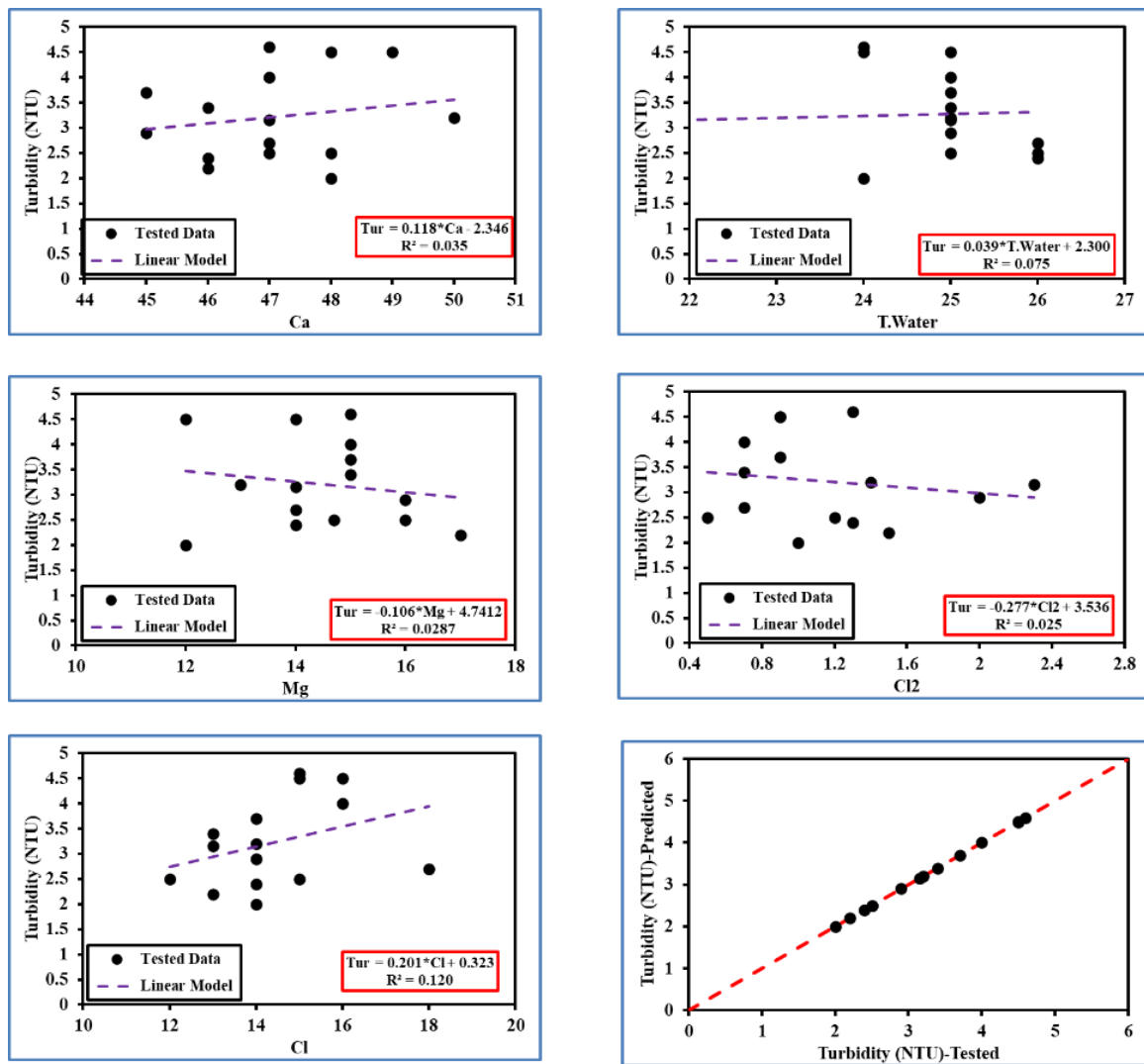
Fig. 10. Correlation of different water quality parameters with turbidity in 2022
