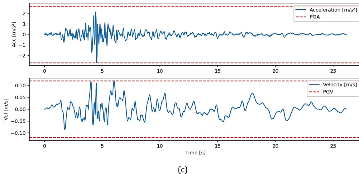
Fig. 5. Acceleration and velocity time histories of the selected earthquake ground motions considered in this study: (a) San Fernando earthquake (1971), (b) Boumerdes earthquake (2003, Dar El Beida station), and (c) Parkfield earthquake (1966)
