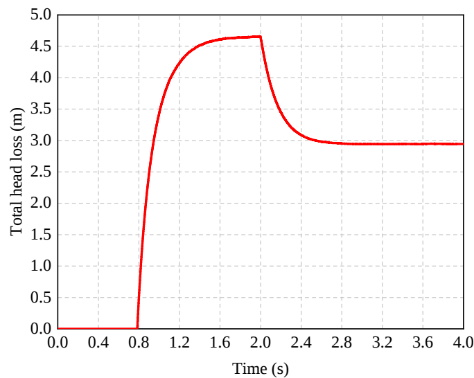
Fig. 19. Total head losses response to an irradiance step ( G: 700 \rightarrow 500 \text{ W/m}^2 )
