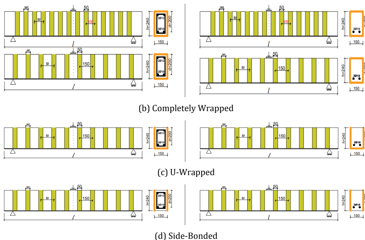
Fig. 1. (a) Geometry and test setup of the test beams; (b), (c), (d) Strengthening configurations
