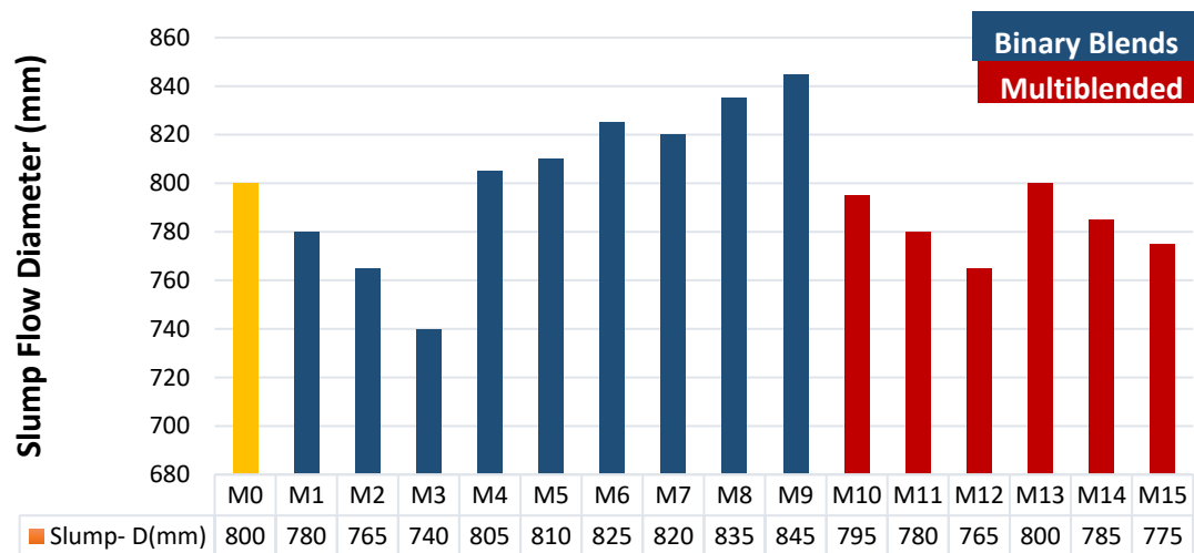
Fig. 5. Slump flow diameter results of HPSCCs
