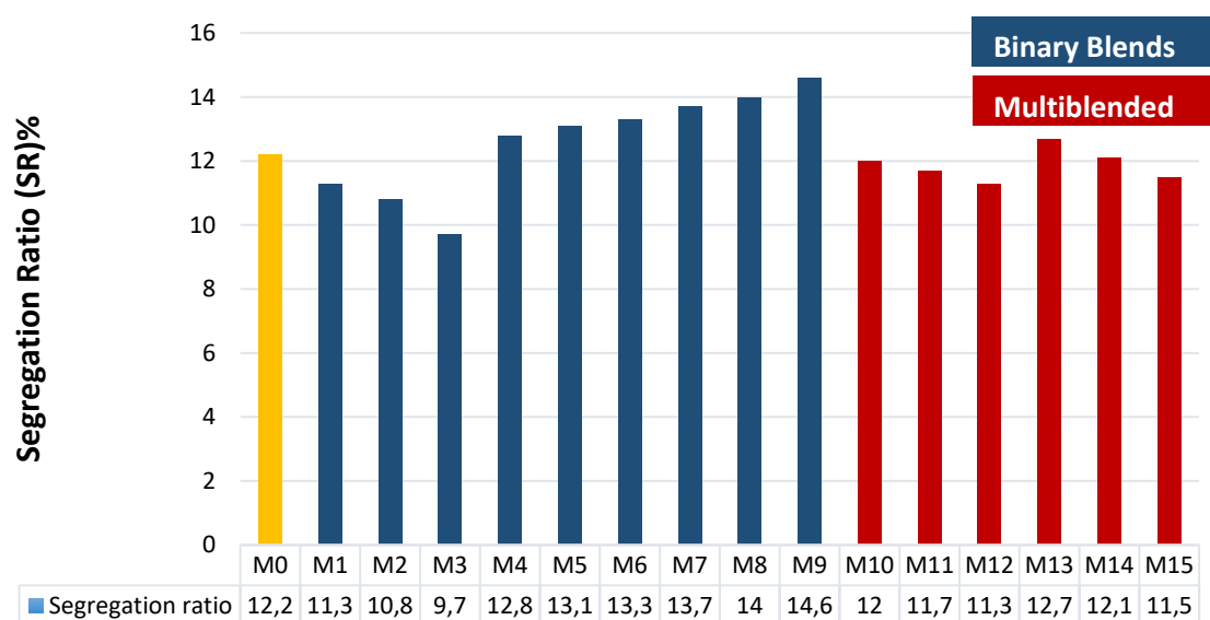
Fig. 7. Segregation ratio results of HPSCCs
