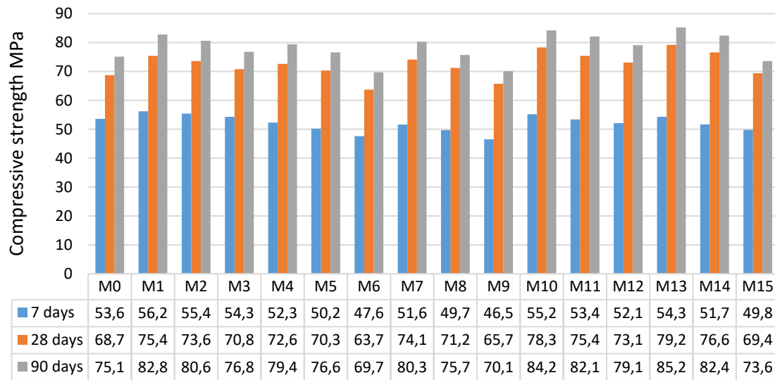
Fig. 10. Development of compressive strength in HPSCCs
