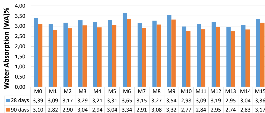
Fig. 12. Water absorption results for binary blends and ternary mixes of HPSCCs
