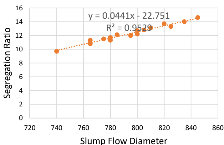
Fig. 8. Relationship between slump flow diameter and segregation ratio of HPSCCs
