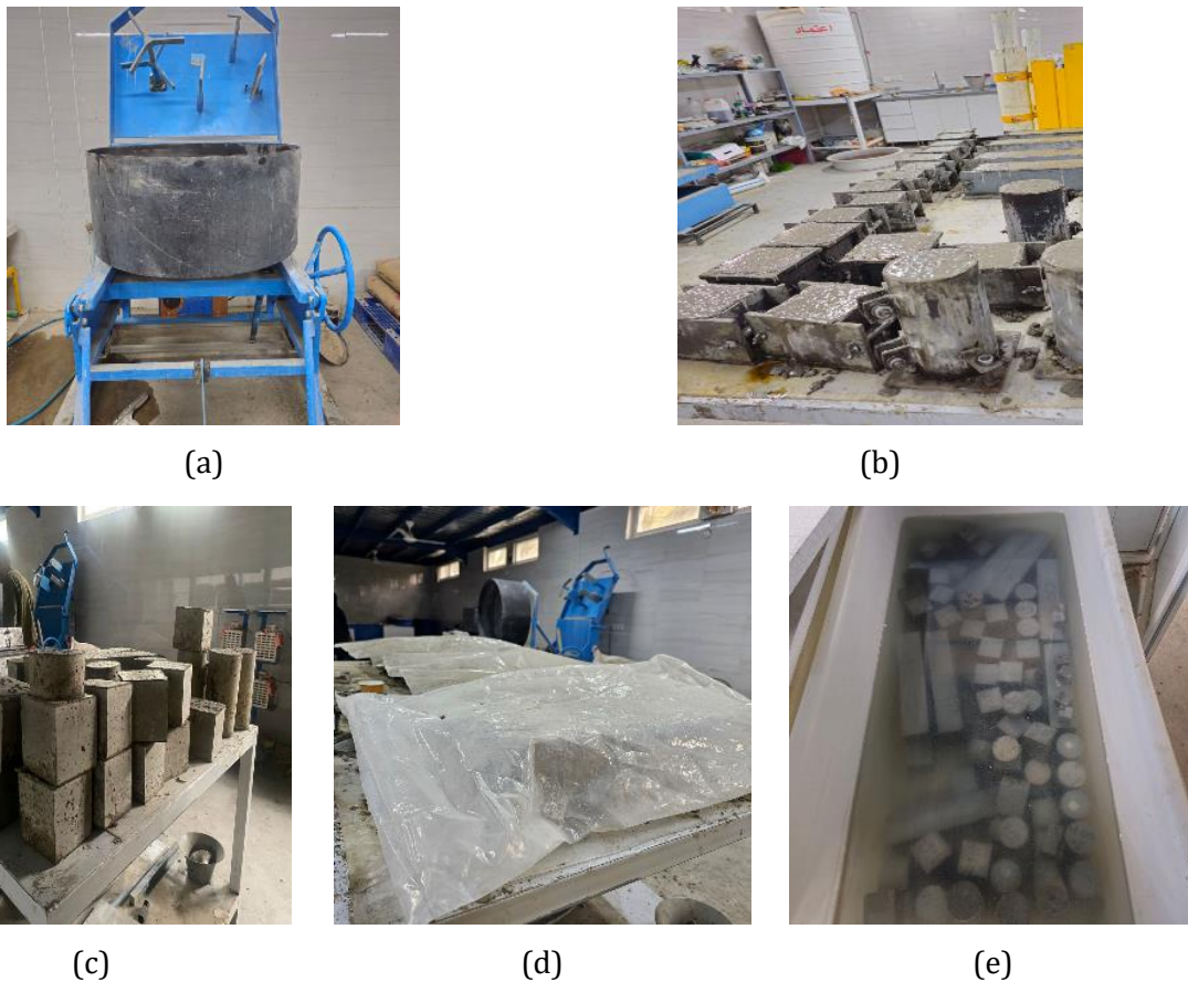
Fig. 2. (a) Mixing (b-d) casting process and (e) curing of test specimens for HPSCC
