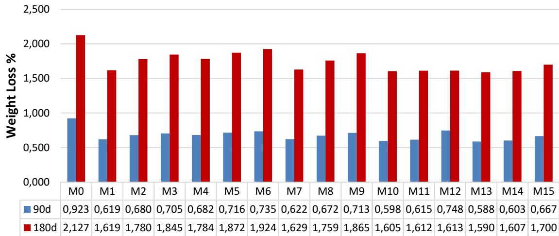
Fig. 13. Weight change results for binary blends and ternary mixes of HPSCCs under chloride (NaCl) exposure at various ages
