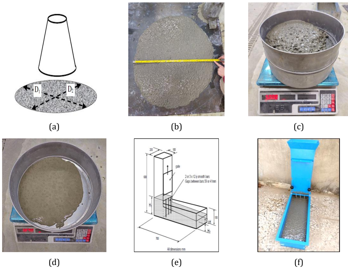
Fig. 3. (a-b) Slump (c-d) sieve segregation resistance and (e-f) L-box tests for HPSCC
