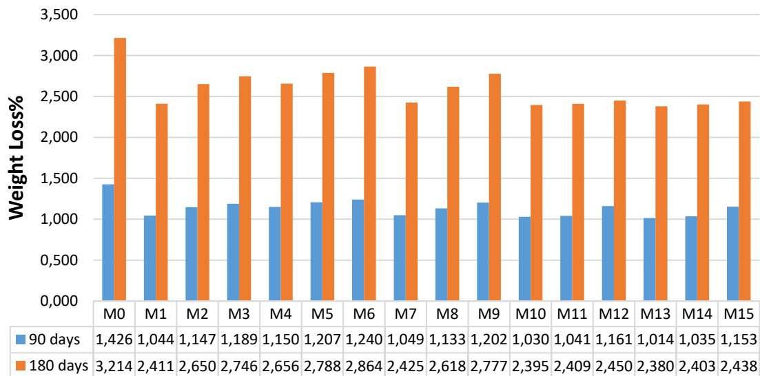
Fig. 14. Weight change results for binary blends and ternary mixes of HPSCCs under sulfate (Na 2 SO 4 ) exposure at various ages
