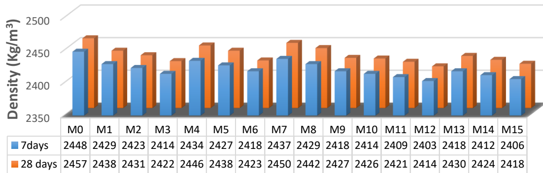
Fig. 9. Density results of HPSCCs
