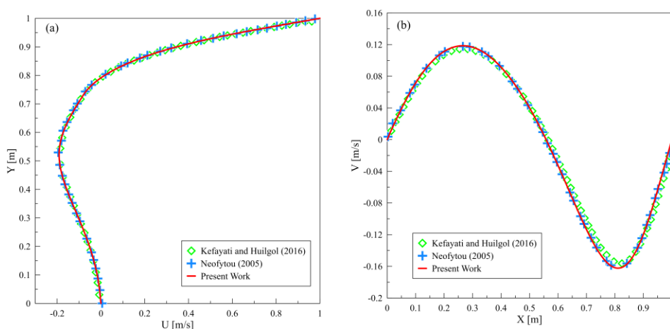
Fig. 2. Velocity profile comparison for model validation: (a) U velocity; (b) V velocity
