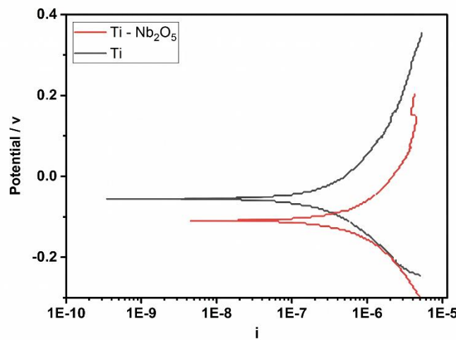
Fig. 3. Electrochemical behavior of Ti and Ti - coated
