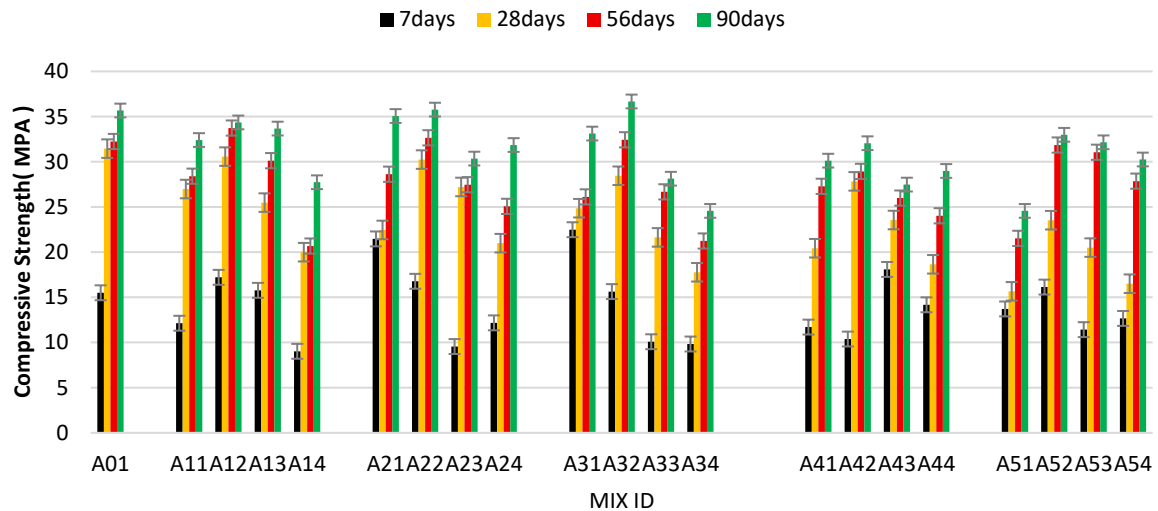
Fig. 5. Compressive strength
