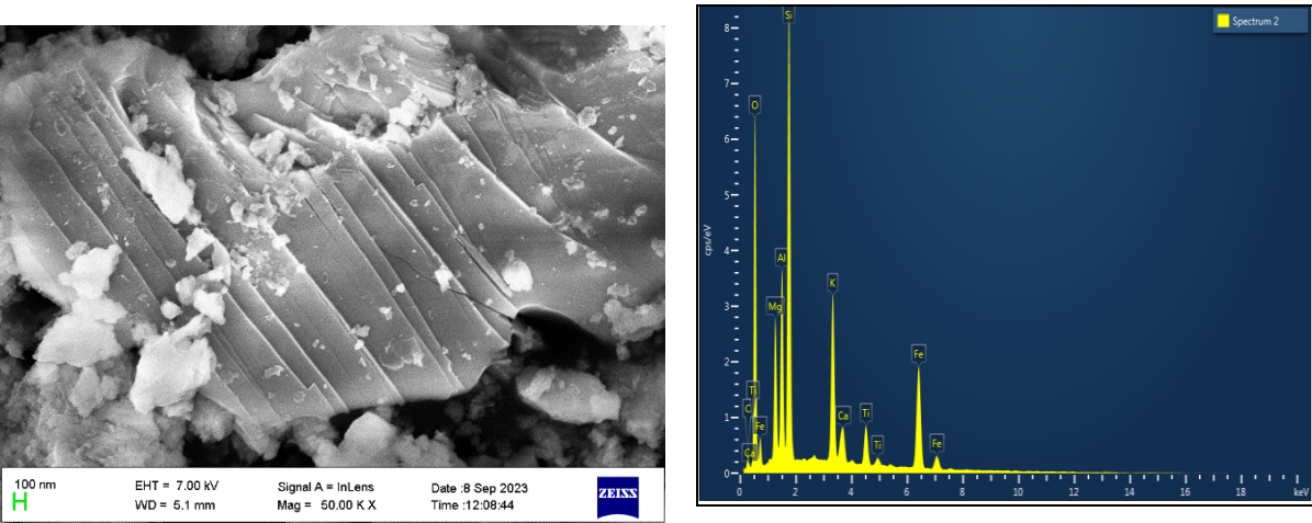
Fig. 18. SEM and EDX image of A22 concrete (20% GGBS and 10% SCBA as binder+5 % SCBA as FA)
