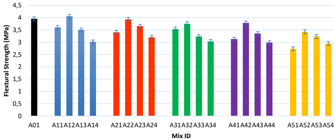
Fig. 7. Flexural strength
