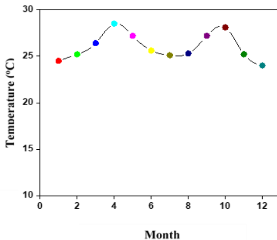
Fig. 1. Shows that the change in average temperature for the period of 12 months
