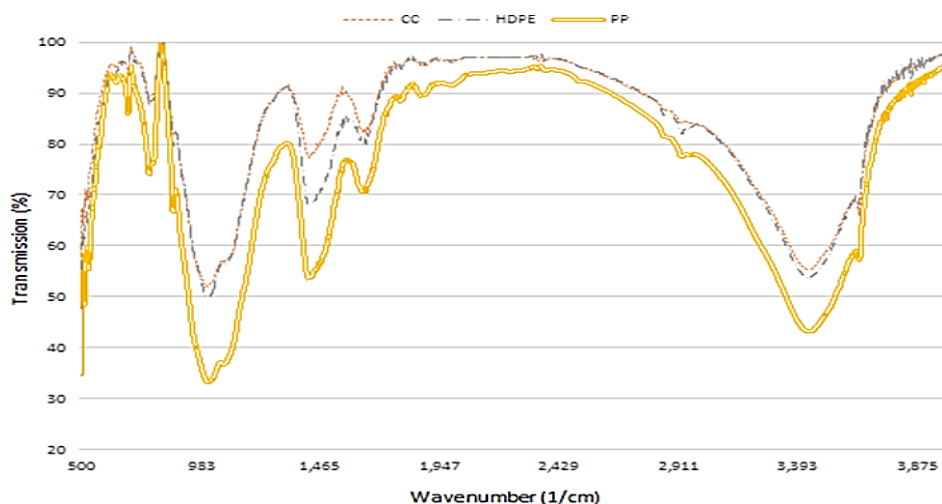
Fig. 7. FTIR analysis of conventional concrete, HDPE, and PP material
