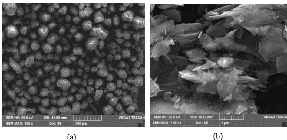
Fig. 1. SEM micrographs of (a) 25-micron sized Al 2 O 3 particles (b) 5 micron sized graphite particles
