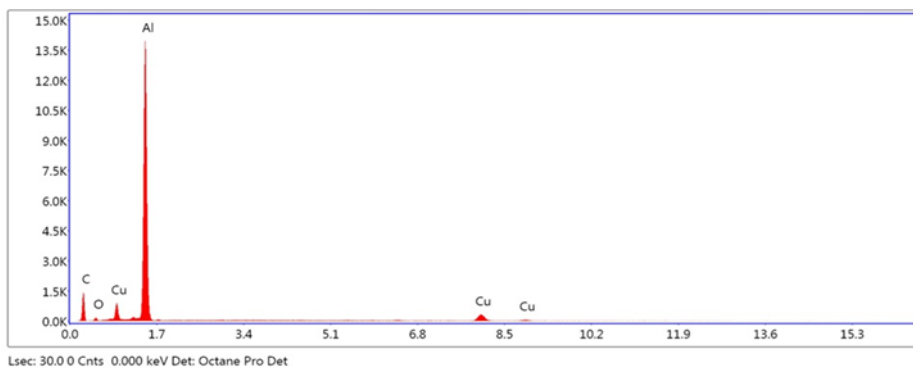
Fig. 4. EDS spectrums of (a) as-cast Al2219 alloy (b) Al2219 alloy with 3 wt. % of \text{Al}_2\text{O}_3 and 2 wt. % of Graphite composite (c) Al2219 alloy with 6 wt. % of \text{Al}_2\text{O}_3 and 2 wt. % of Graphite composite
