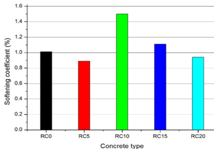
Fig. 11. Softening coefficient at 60 days
