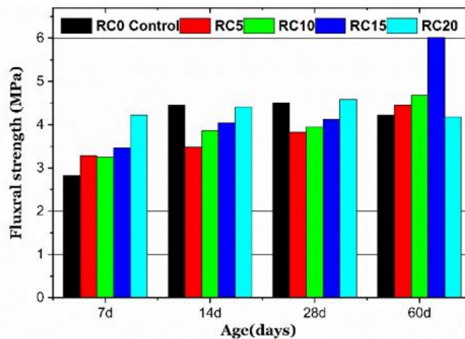
Fig. 8. Flexural strength of different RAC formulations and marble fines
