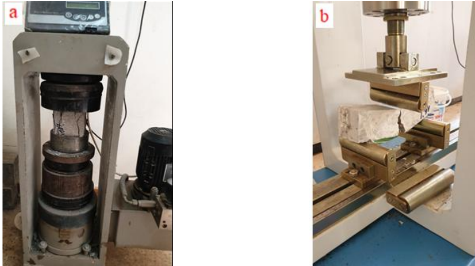
Fig. 6. (a) Compressive strength testing of concrete, (b) Flexural strength testing of concrete
