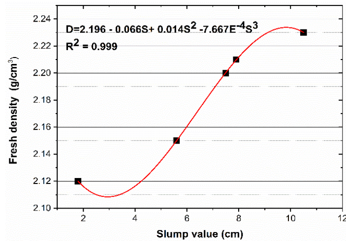
Fig. 14. Relationship between fresh density and slump of RAC with and without marble fines
