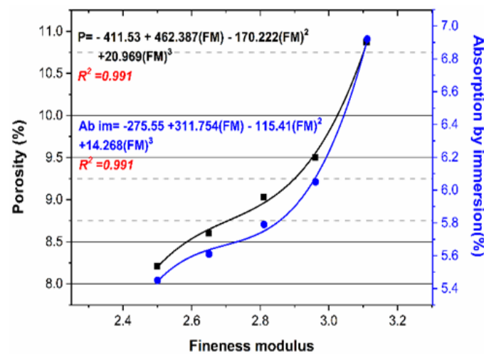
Fig. 15. Relationship between porosity, absorption by immersion and fineness modulus of RAC with and without marble fines
