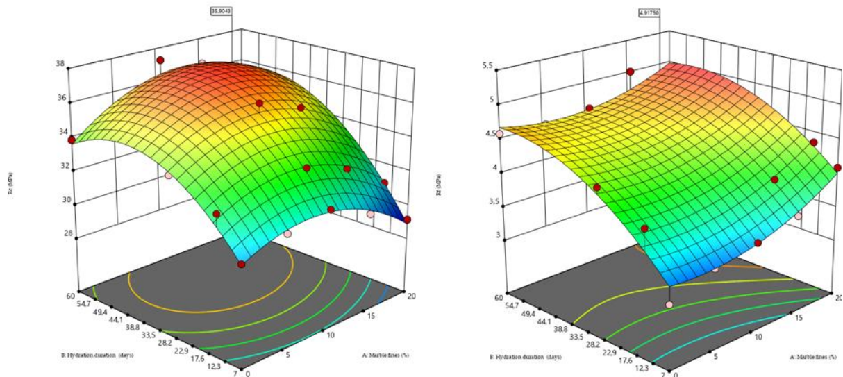
Fig. 19. 3D response surface representation RSM models for R_c and R_f
