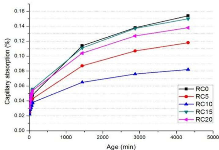
Fig. 9. Capillary water absorption values at 60 days of recycled demolition concrete with and without marble fines as a function of time
