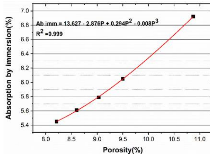
Fig. 16. Relationship between absorption by immersion and porosity of RAC with and without marble fines
