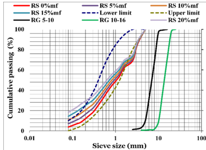
Fig. 3. Particle size analysis of studied aggregates
