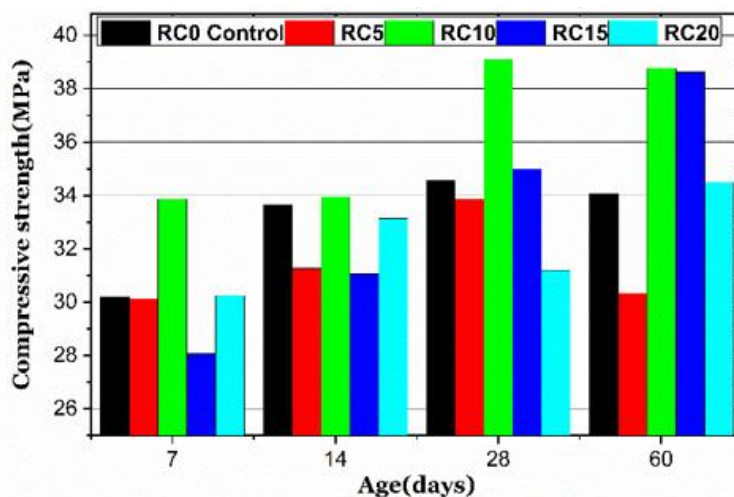
Fig. 7. Compressive strength of different RAC formulations and marble fines
