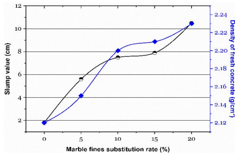
Fig. 5. Effect of marble fines incorporation rate on fresh concrete's workability and density
