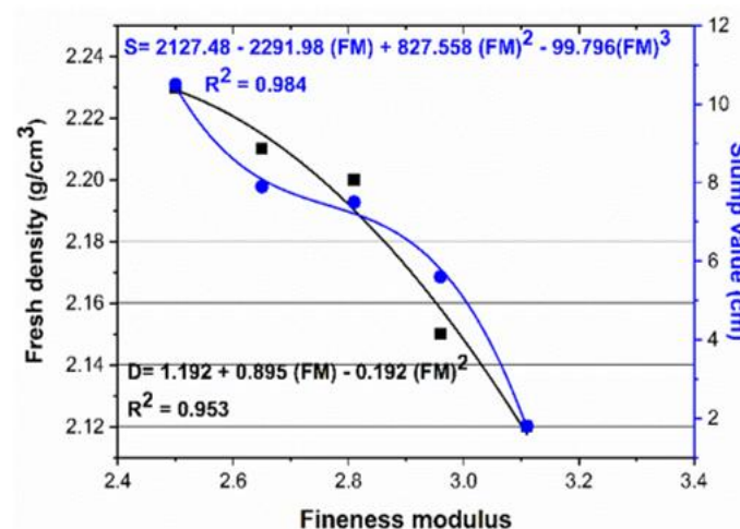
Fig. 13. Relationship between fresh density, slump and fineness modulus of RAC with and without marble fines
