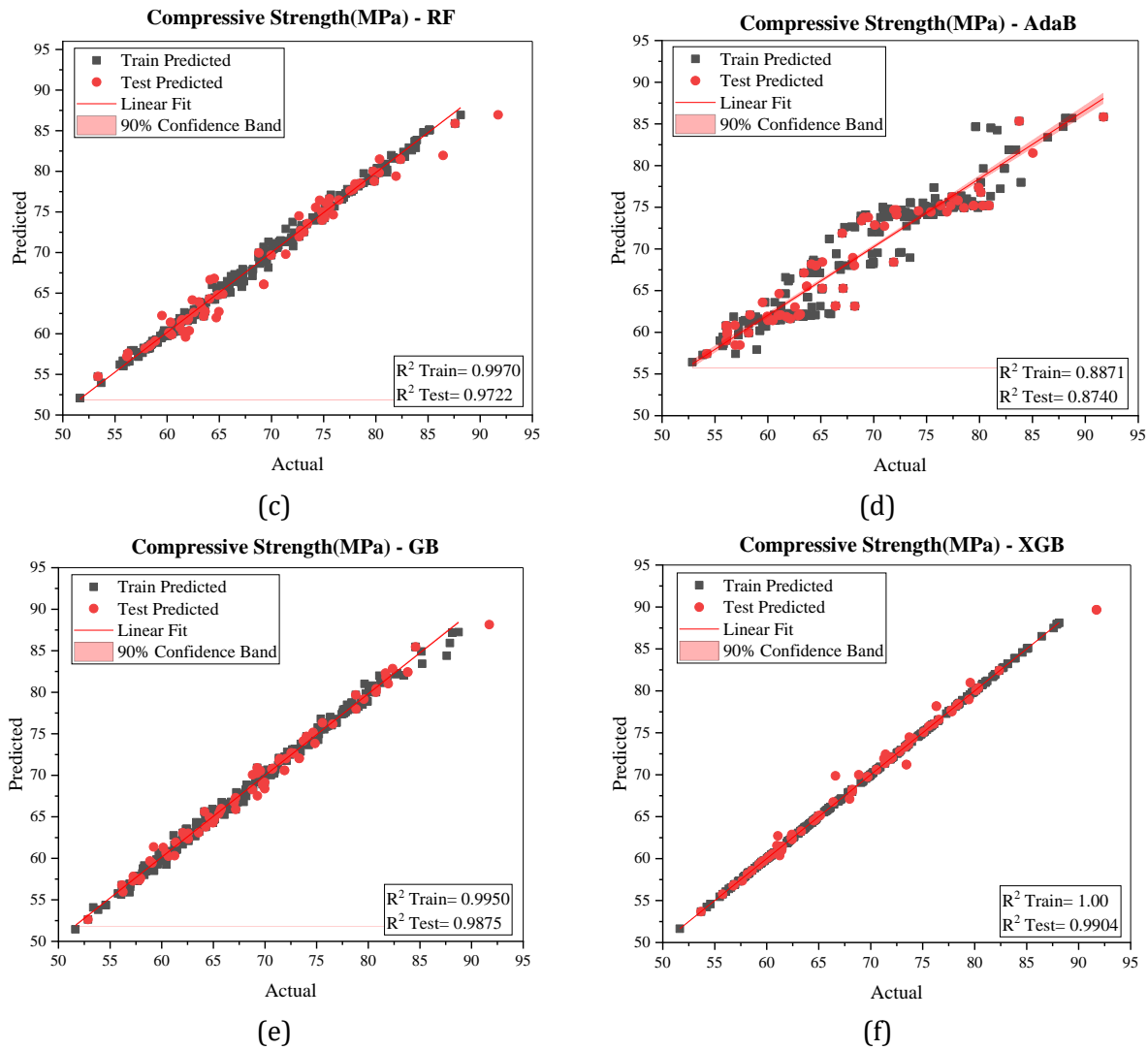
Fig. 11. Parity plots comparing experimentally and predicted compressive strength of MSHPC using different models: (a) ANN, (b) NLR, (c) RF, (d) AdaB, (e) GB, and (f) XGB
