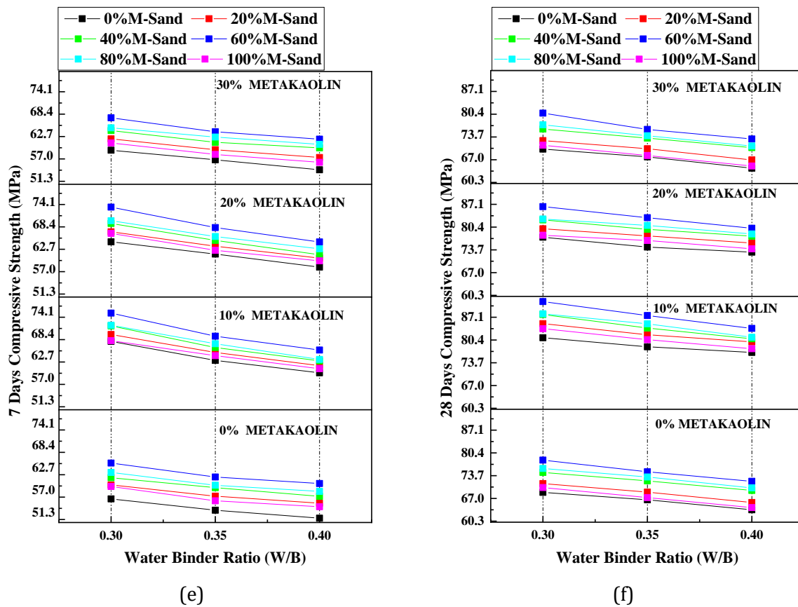
Fig. 2. Compressive strength vs W/B Ratio: (a) FA: 7-day CS vs W/B, (b) FA: 28-day CS vs W/B, (c) SF: 7-day CS vs W/B, (d) SF: 28-day CS vs W/B, (e) MK: 7-day CS vs W/B, and (f) MK: 28-day CS vs W/B.
