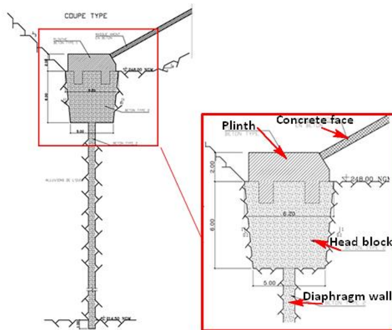
Fig. 2. Typical section of the diaphragm wall (adapted from [1])
