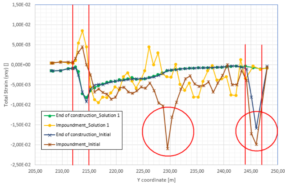
Fig. 13. Focus on last phases curves of the displacements
