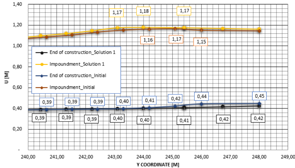
Fig. 12. Focus on last phases curves of the displacements
