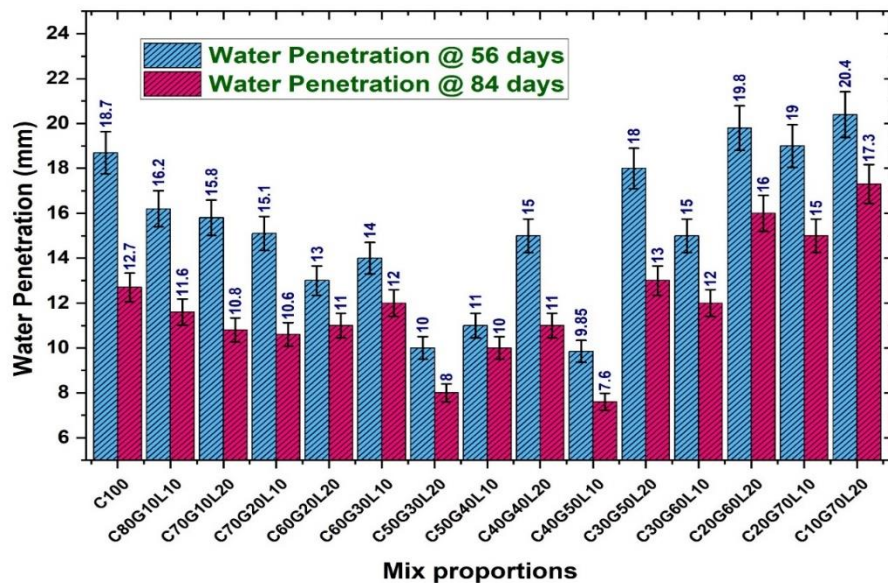
Fig. 3. Combined influence of HL and GGBS on the water penetration characteristics
