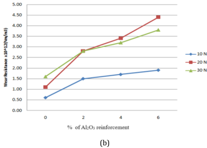
Fig. 8. (a)Wear loss and 7(b) Wear Resistance of nitride (Al-5%Ti-B) materials with 0%, 2%, 4% and 6% of reinforced Al 2 O 3
