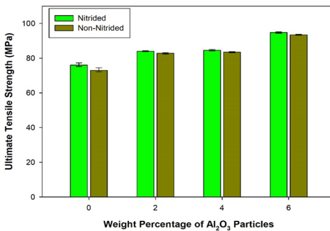
Fig. 5. Nitrated and Non- Nitrated Tensile strength of (Al-5%Ti-B) materials with 0%, 2%, 4% and 6% of reinforced \text{Al}_2\text{O}_3
