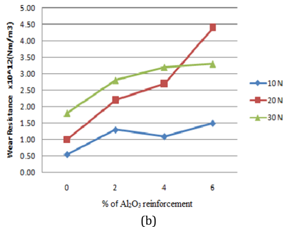
Fig. 7.(a) Wear loss and 7and (b) Wear Resistance of non Nitrided (Al-5%Ti-B) materials with 0%, 2%, 4% and 6% of reinforced Al 2 O 3
