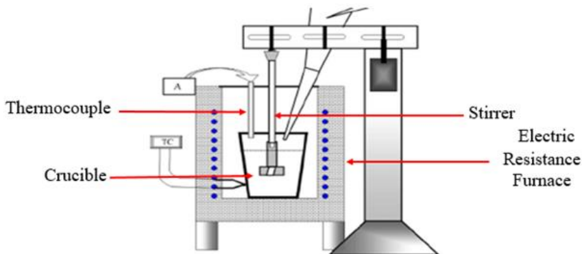
Fig. 1. The schematic diagram of the furnace used for composite ingot preparation
