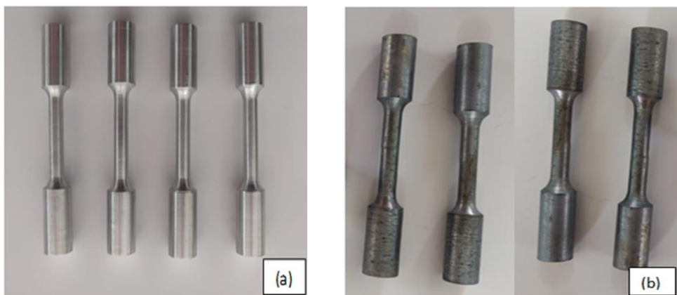
Fig. 4. (a) Non-Nitrated Tensile specimen and (b) Nitrated Tensile specimen as per ASTM standard with 0%, 2%, 4% and 6% of reinforced \text{Al}_2\text{O}_3
