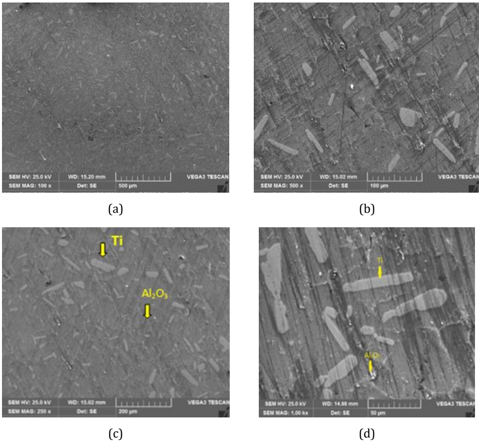
Fig. 3. SEM result of (a-b) Al-5%Ti-B composition (c-d) Al-5%Ti-B composition reinforced with \text{Al}_2\text{O}_3
