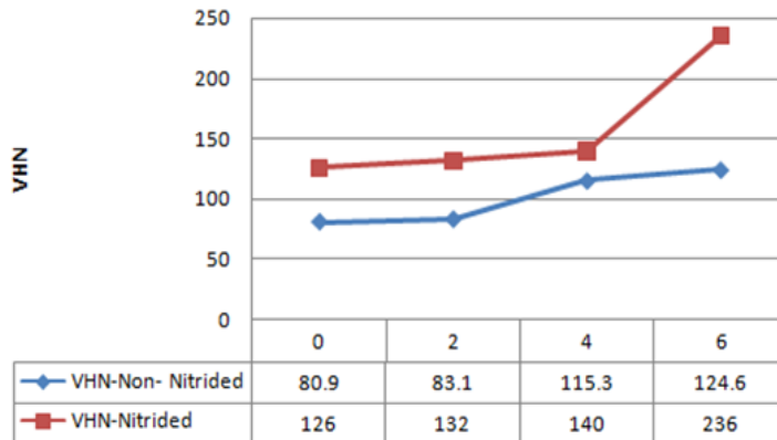
Fig. 6. Nitrided and Non- Nitrided Vicker's hardness of (Al-5%Ti-B) materials with 0%, 2%, 4% and 6% of reinforced \text{Al}_2\text{O}_3
