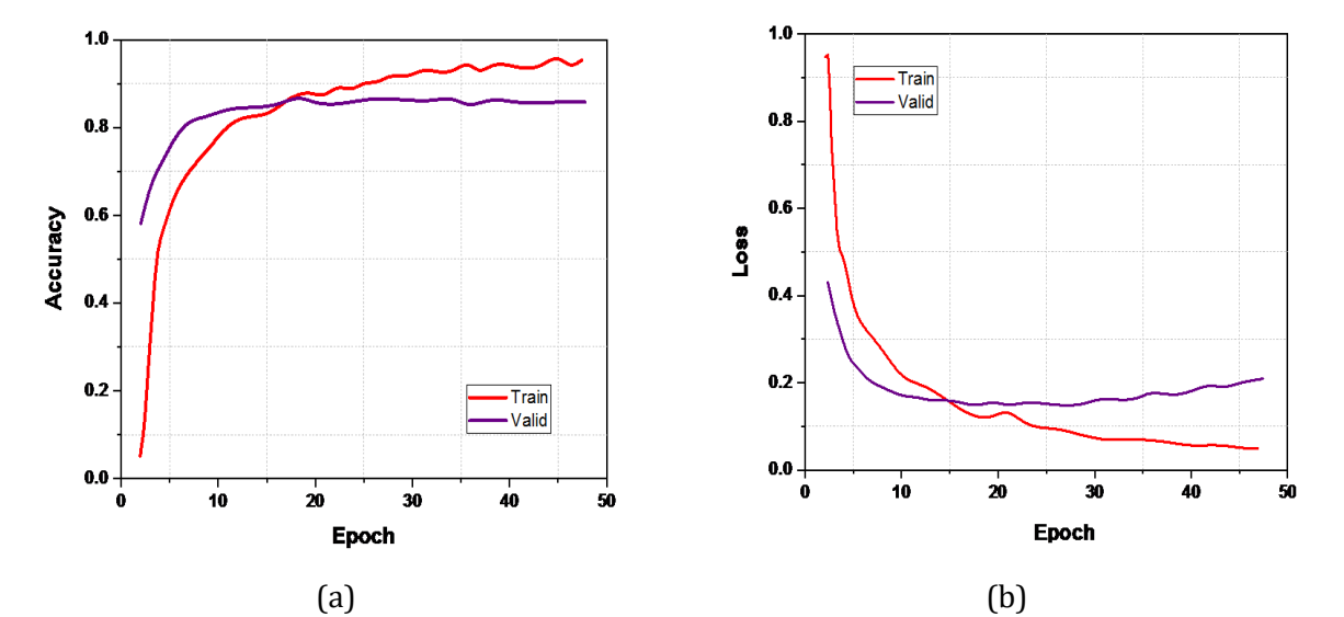
Fig. 2. a) Accuracy and b) Loss
