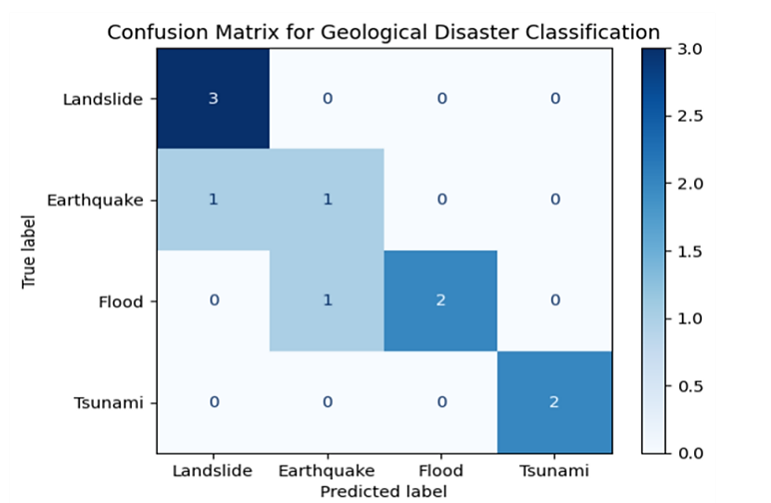
Fig. 3.: Confusion matrix
