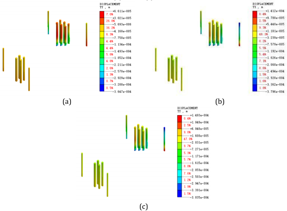
Fig. 9. Y-direction displacements of pedestrian bridge pile infrastructure in (m) using initial support construction and excavation of escalator sections at subway entrance and exit (a) case 1 (b) case 2 (c) case 3
