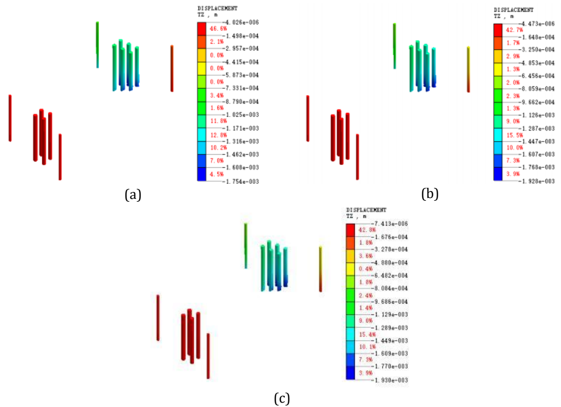
Fig. 11. Z-direction displacements of pedestrian bridge pile infrastructure in (m) using initial support construction and excavation of escalator sections at subway entrance and exit (a) case 1 (b) case 2 (c) case 3
