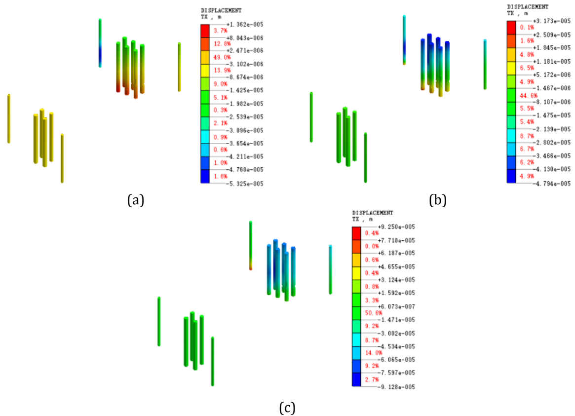
Fig. 6. X-direction displacements of pedestrian bridge pile infrastructure in (m) using initial support construction and excavation of subway entrance and exit straight sections (a) case 1 (b) case 2 (c) case 3
