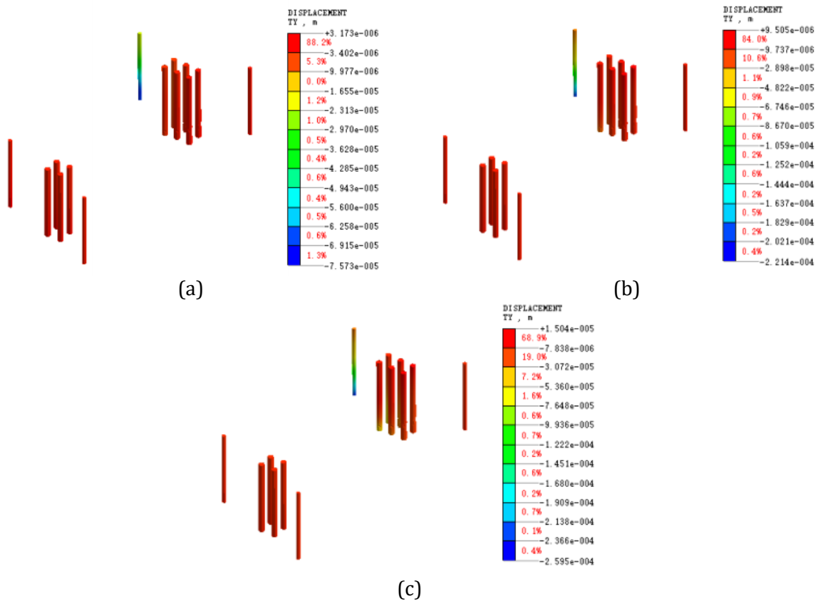
Fig. 8. Y-direction displacements of pedestrian bridge pile infrastructure in (m) using initial support construction and excavation of subway entrance and exit straight sections (a) case 1 (b) case 2 (c) case 3
