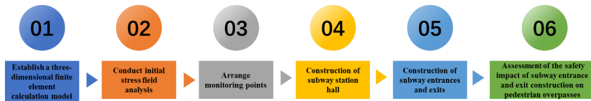
Fig. 5. Research flowchart
