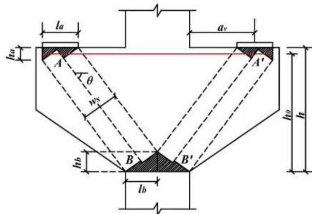
Fig. 15. Strut and tie model for symmetrical two-sided corbel [67]
