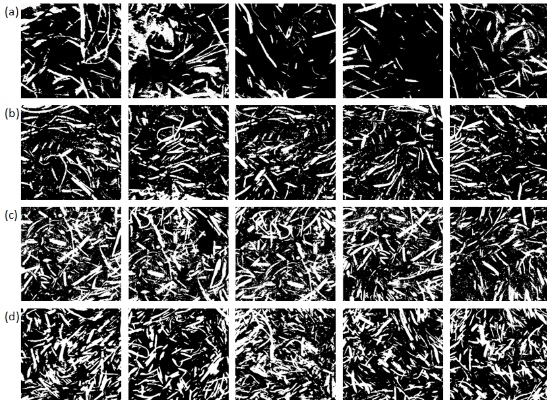
Fig. 16. Realizations of microstructure for RVE' size 1000×1000 pixels, and weight fractions of fibres: (a) W_f = 10\% , (b) W_f = 15\% , (c) W_f = 20\% , and (d) W_f = 25\%
