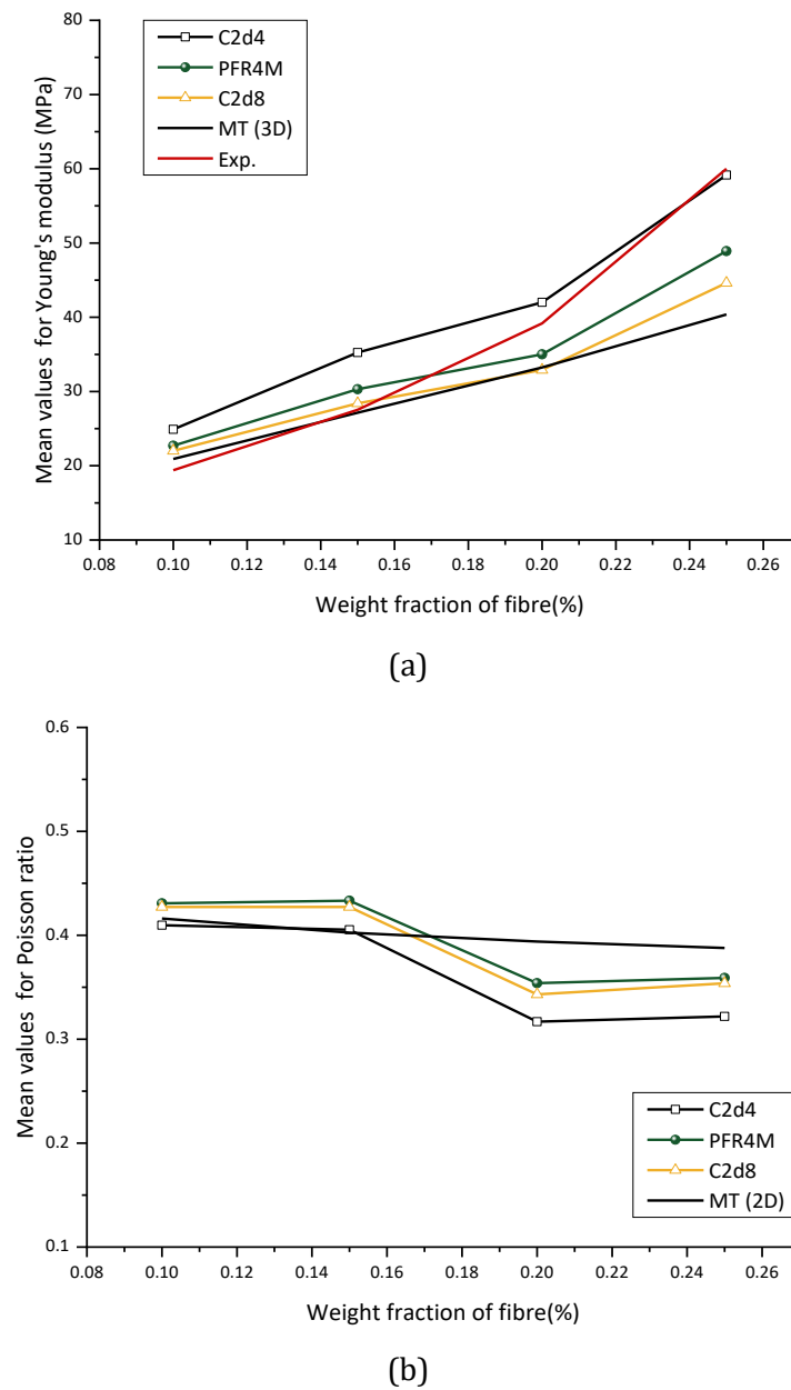
Fig. 14. Mechanical properties versus weight fraction. (a) Longitudinal Young's modulus. (b) Poisson ratio
