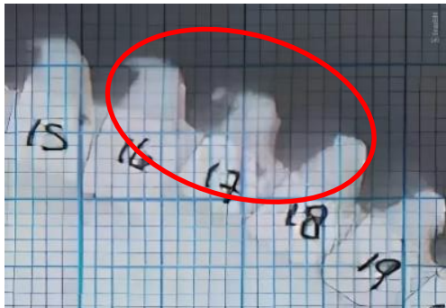
Gear damage under lubricated conditions (c) After 120 \times 10^4 cycles for drive gear
