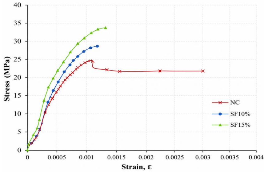
Fig. 10. Compressive stress–strain responses of NC, SF10, and SF15 obtained from instrumented cylinder tests
