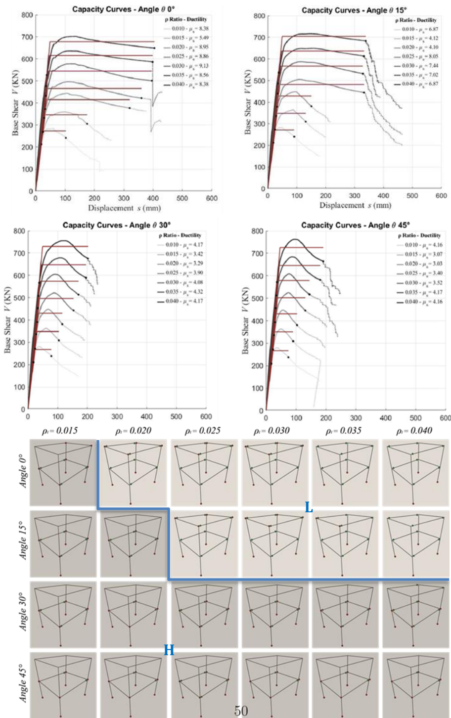
Fig. 7. Failure mechanisms in model T2 for different values of longitudinal reinforcement ratio and angles of attack. Red and green dots: plastic hinges in columns and beams, respectively. Dark and light grey background: "H" and "L" mechanism, respectively
