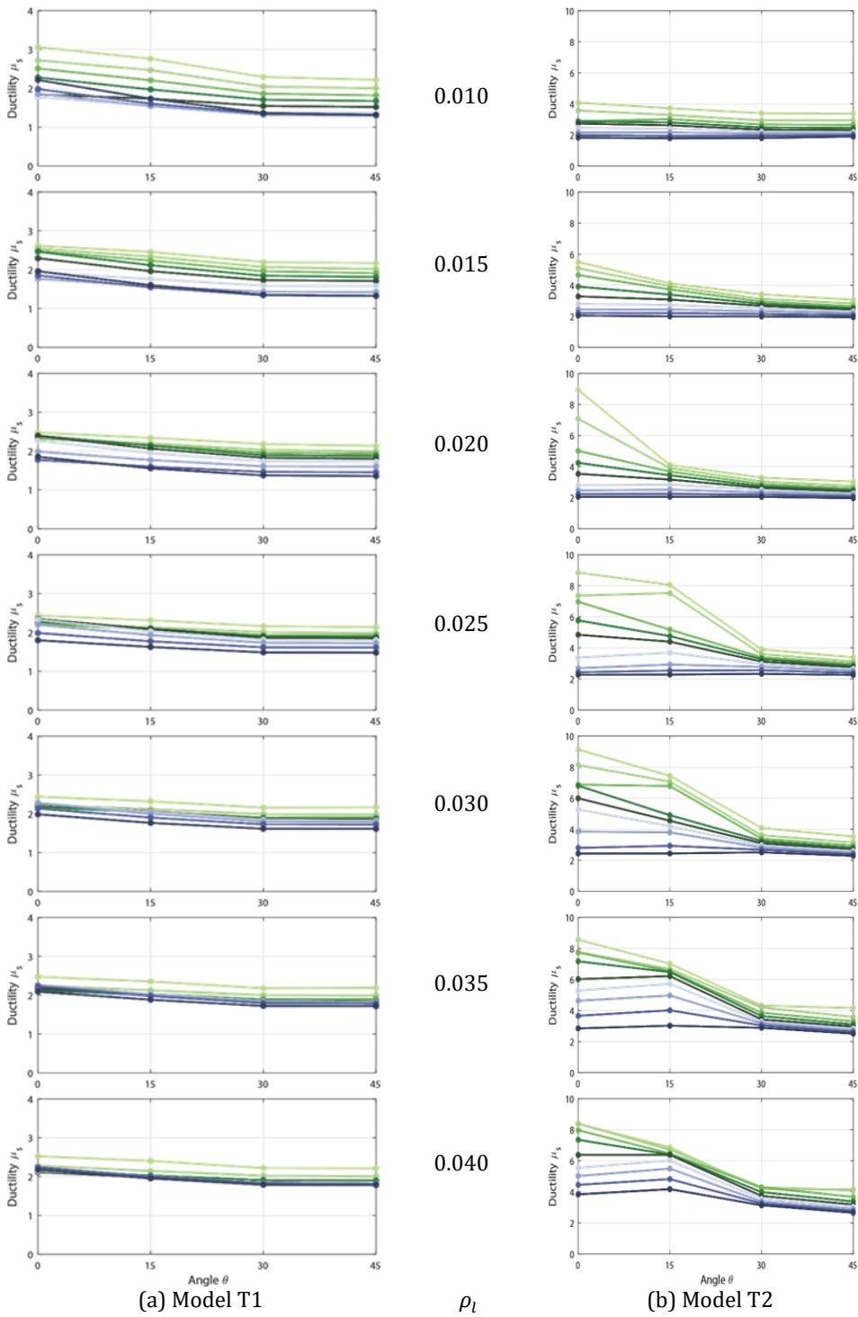
Fig. 6. Ductility values \mu_s obtained for \omega_{wd}=0.28 and different values of \rho_l (from 0.010 at the top to 0.040 at the bottom) and v (from 0.10 depicted with light green to 0.50 represented with dark blue) for model T1 (a) and model T2 (b)
