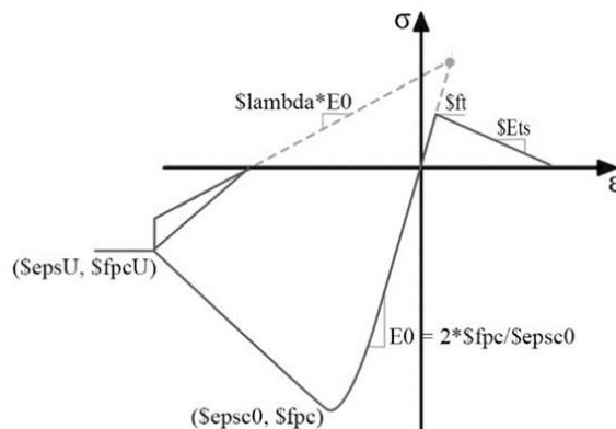
Fig. 2. Hysteretic Stress-Strain Relation for Concrete02 materials
