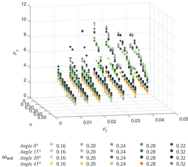
Fig. 5. Complete plot of displacement ductility factors for model T2
