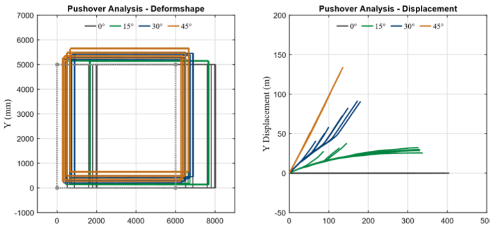
Fig. 8. Planar positions (left) and displacements of the control point (right) at the end of pushover analysis for model T2
