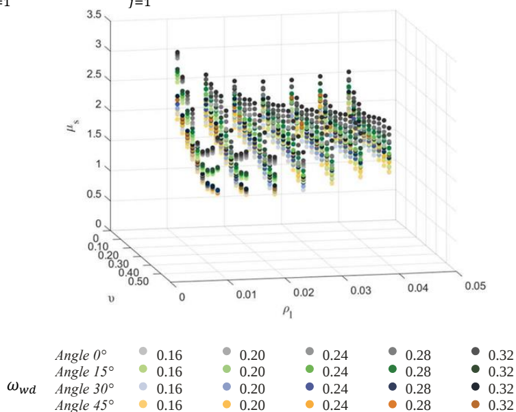
Fig. 4. Complete plot of displacement ductility factors for model T1
