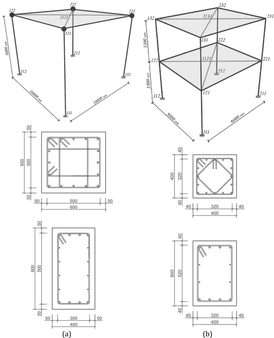
Fig. 1. Perspective view with main dimensions, cross sections and reinforcements of columns and beams (from top to bottom) for (a) model T1 and (b) model T2
