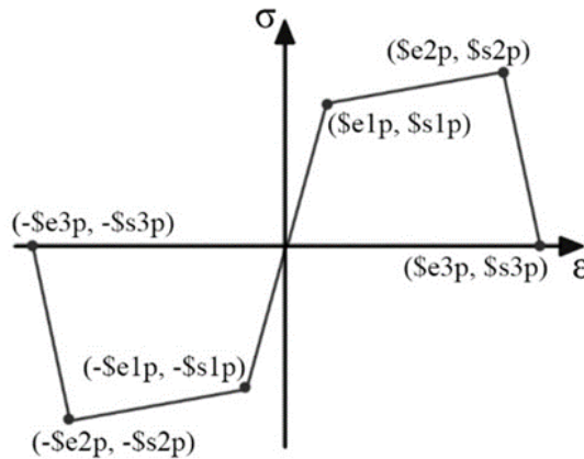
Fig. 3. Hysteretic Stress-Strain Relation for steel rebars
