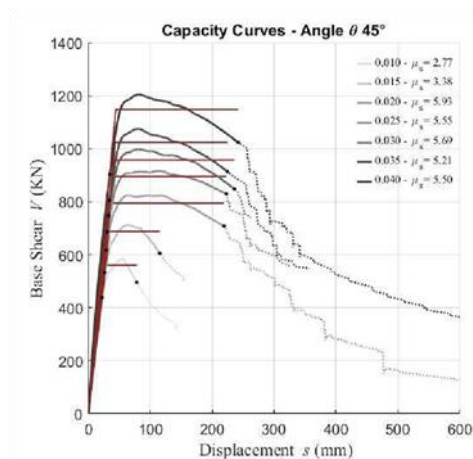
Fig. 11. Capacity curves of model T2 with 500×500 mm cross section columns
