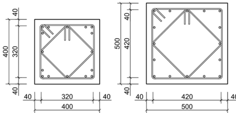
Fig. 9. Section 400×400 mm with improved steel rebars distribution (left) and section 500×500 mm satisfying Eq. (21)
