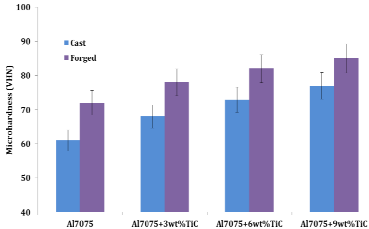
Fig. 5. Variation of hardness with TiC reinforcement for cast and forged
