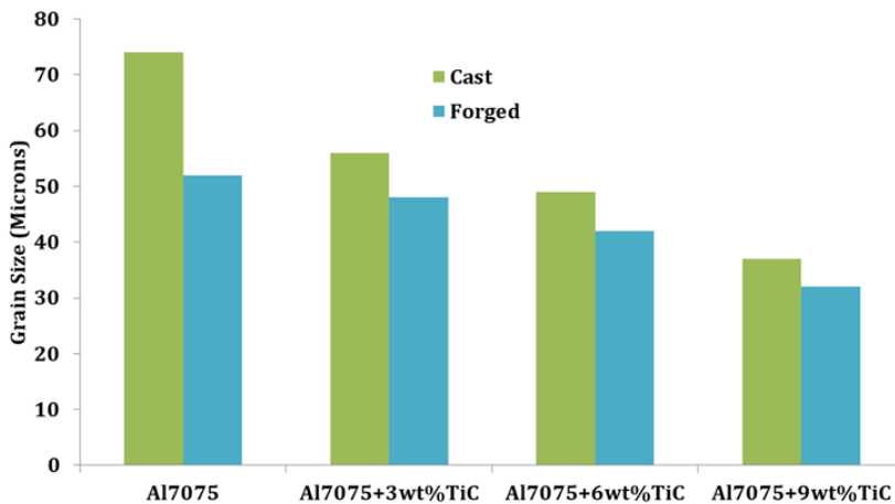
Fig. 4. Variation of grain size with TiC reinforcement for cast and forged composites
