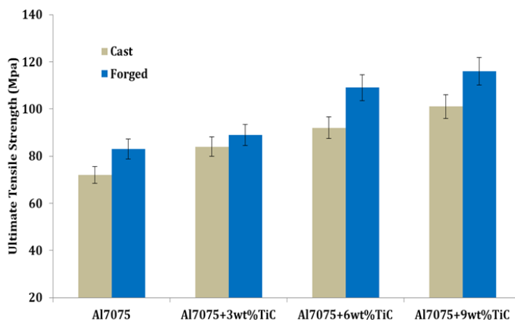
Fig. 6. Variation of UTS with TiC reinforcement for cast and forged composites
