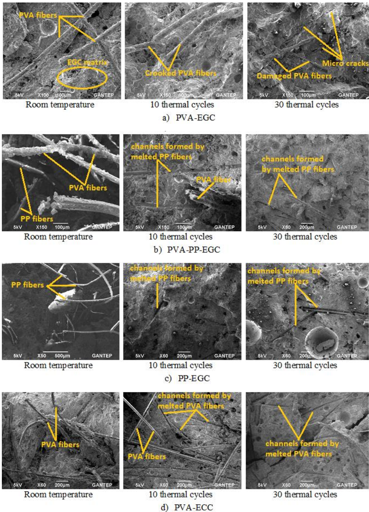
Fig. 3. SEM images of the green LW (ECC and EGC) composites both before and after being subjected to heating-cooling cycles
