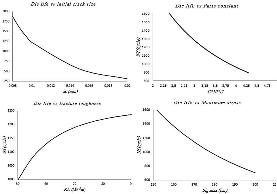
Fig. 4. Variation of die life against geometrical parameters
