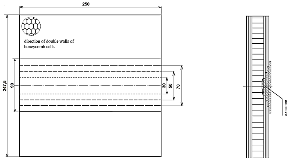
Fig. 2. Scheme of the arrangement of layers of the repair patch
