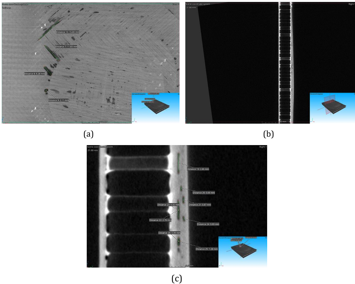
Fig. 9. Results of tomography of the patch of zone 2, performed by vacuum method with excess pressure (a) - Cross-section of the repair patch of zone 2; (b) - General view of the side section of the repair patch of zone 2; (c) - General view of the side section of the repair patch of zone 2
