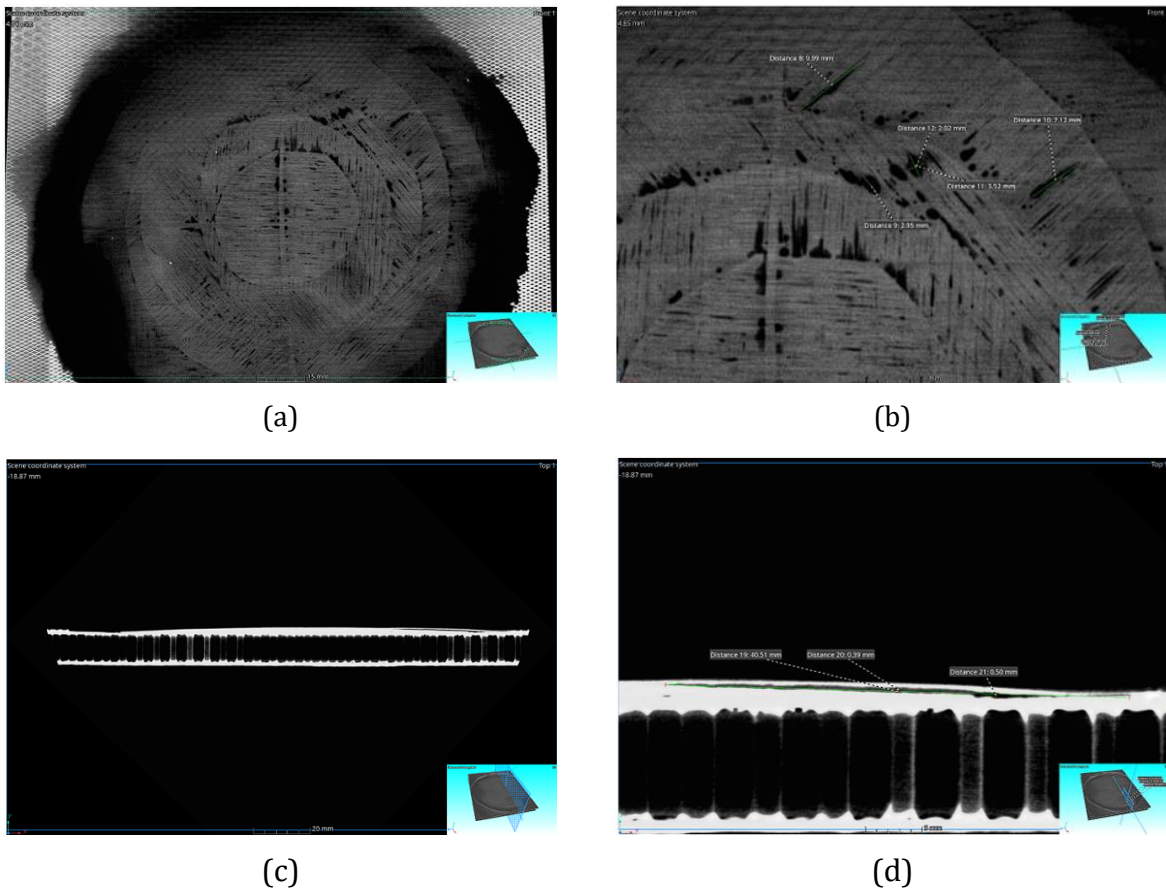
Fig. 11. Results of tomography of the patch of zone 3, performed by vacuum method with exceeding curing temperature (a) - Cross-section of the repair patch of zone 3; (b) - Local area of the cross-section of the repair patch; (c) - General view of the side section of the repair patch of zone 3; (d) - Local area of the side section of the repair patch with extensive delamination
