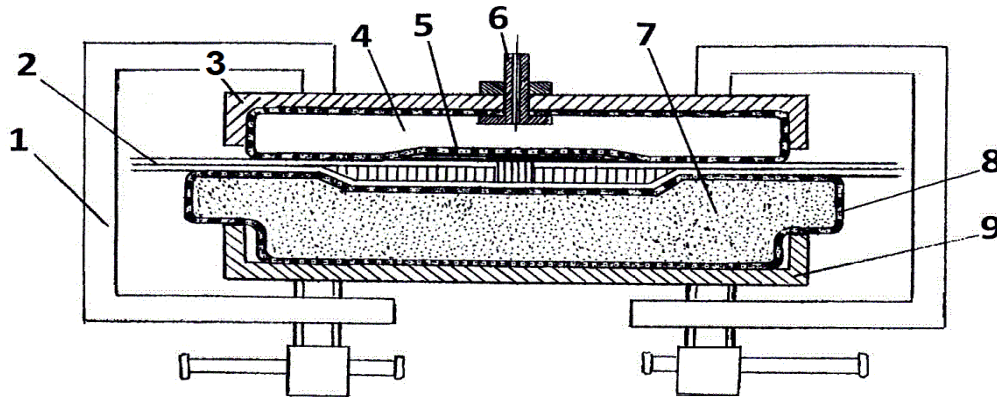
Fig. 4. Scheme of providing excess pressure during repair: 1 - clamp; 2- repaired structure; 3- air bag box; 4- air bag; 5- repair zone; 6- fitting for compressed air supply; 7- sand; 8- shell of the sand-filled bag; 9- the sand-filled bag supports
