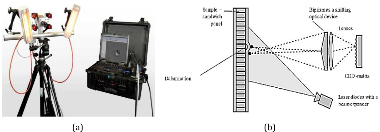
Fig. 5. Apparatus of shearography system(a) - System with automatic loading by heating; (b) - The principle of the shearograph's operation
