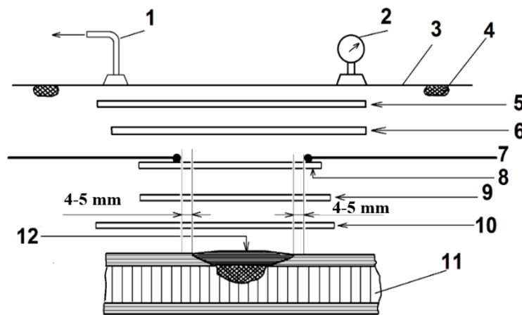
Fig. 3. Assembly scheme of the vacuum bag: 1- air suction; 2- device for controlling the suction in the vacuum bag; 3- vacuum bag shell; 4- sealing gasket; 5- vacuum bag's drainage layer (padding polyester, fiberglass); 6- heater (thermal blanket); 7- thermocouple; 8- non-perforated separating film; 9- layers of fabric absorbing excess resin (glue) – nylon or polyethylene terephthalate; 10- perforated separating film; 11- repaired structure; 12- repair patch layers in the repair zone
