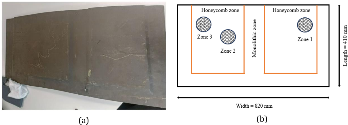
Fig. 1. Repair three-layer carbon fiber honeycomb panel (a) External appearance of the panel (top view); (b) Schematic view of the repair panel with marked repair zones and overall dimensions
