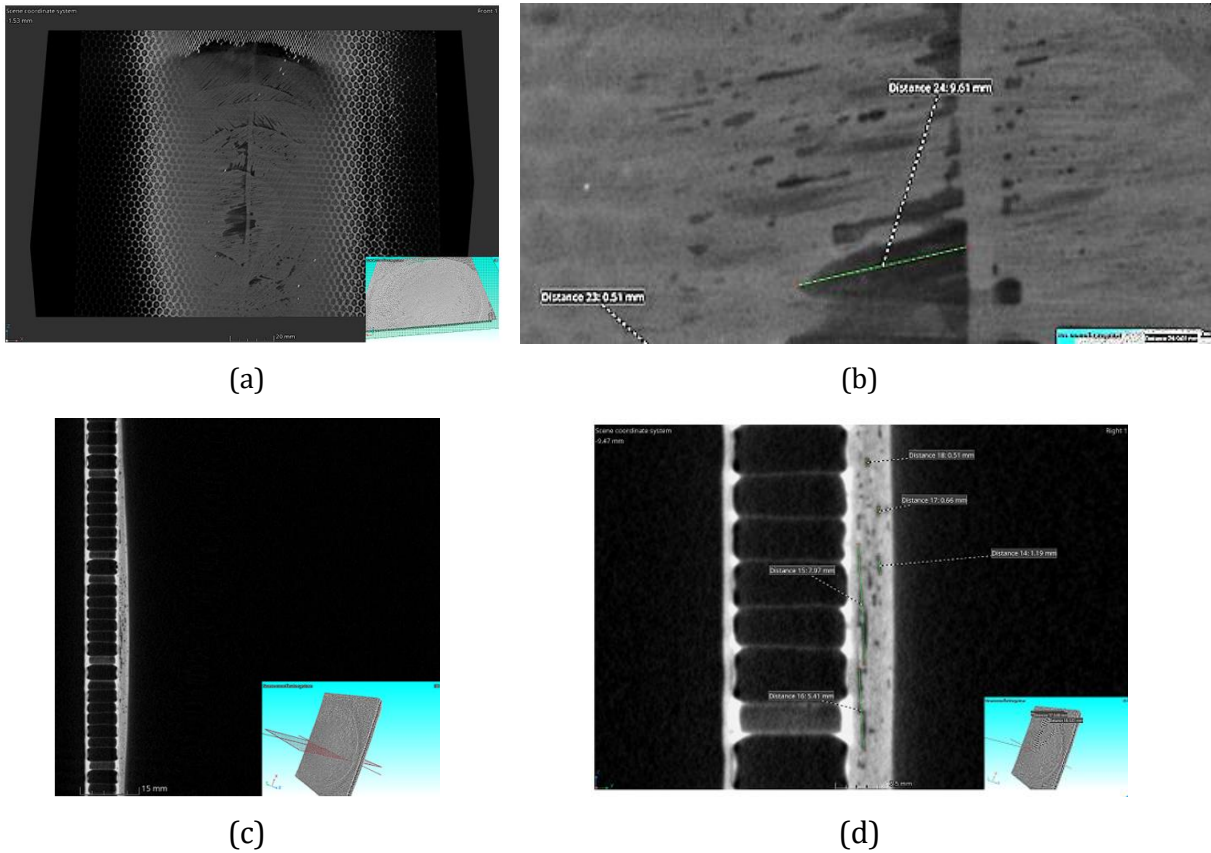
Fig. 7. Results of tomography of repair zone 1, performed by vacuum method(a) General view of the repair patch section; (b) Local repair patch section zone; (c) Side section of the repair patch; (d) Local zone of the side section of the repair patch
