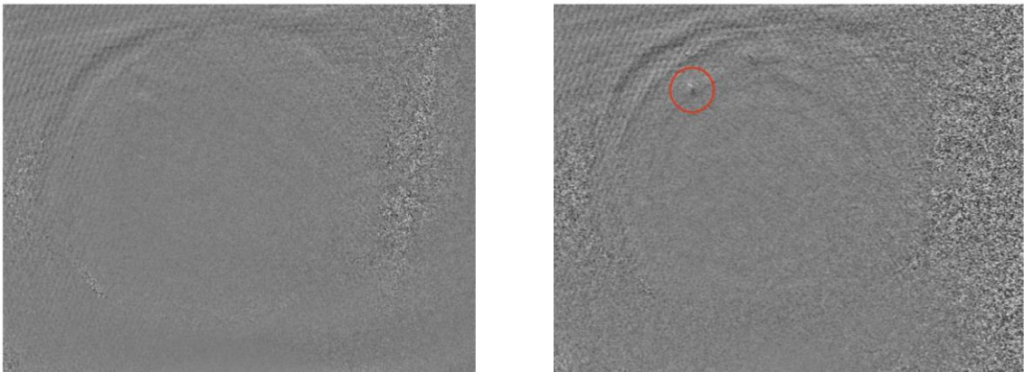
Fig. 12. Shearograms of the patch performed by vacuum method
