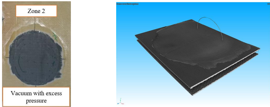
Fig. 8. Repair patch in zone 2, performed by vacuum method with excess pressure
