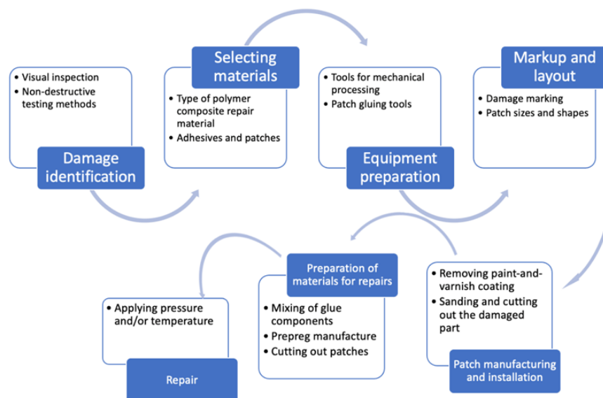
Fig. 1. Overall repair procedure flowchart
