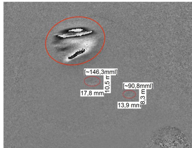
Fig. 14 – Shearograms of the patch obtained using vacuum and exceeding curing temperature
