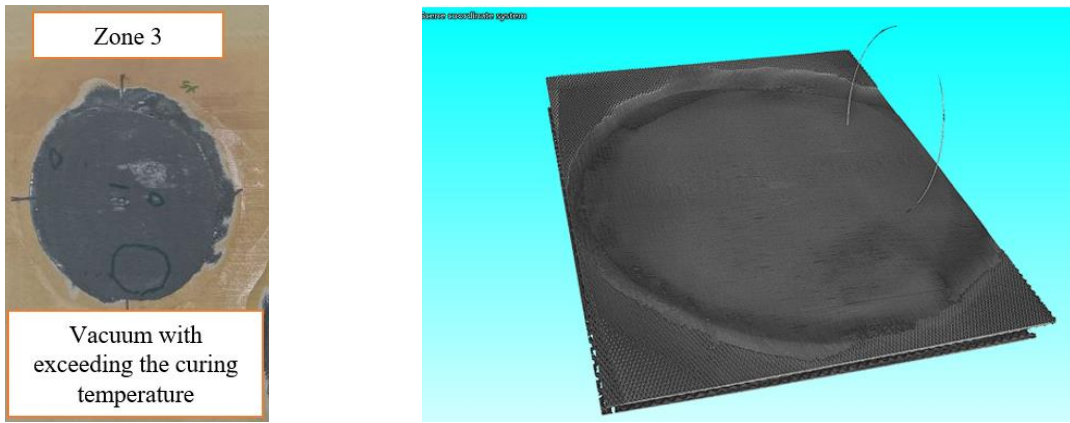
Fig. 10. Repair patch in zone 3
