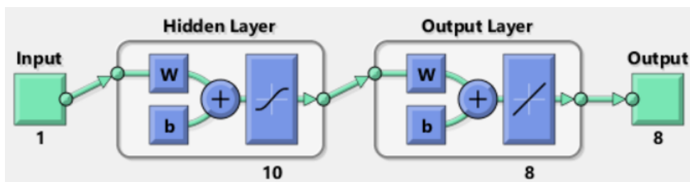
Fig.11. Architecture of the ANN model with one hidden and output layer
