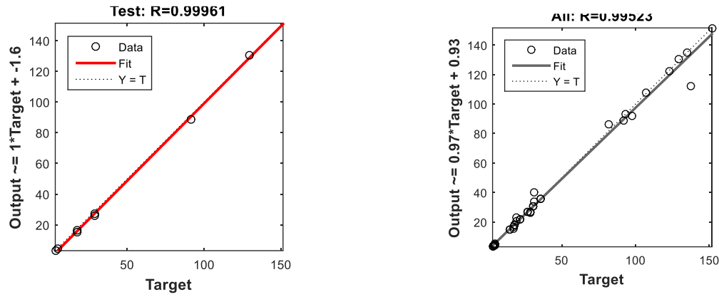
Fig. 15. Model performance evaluation through regression analysis
