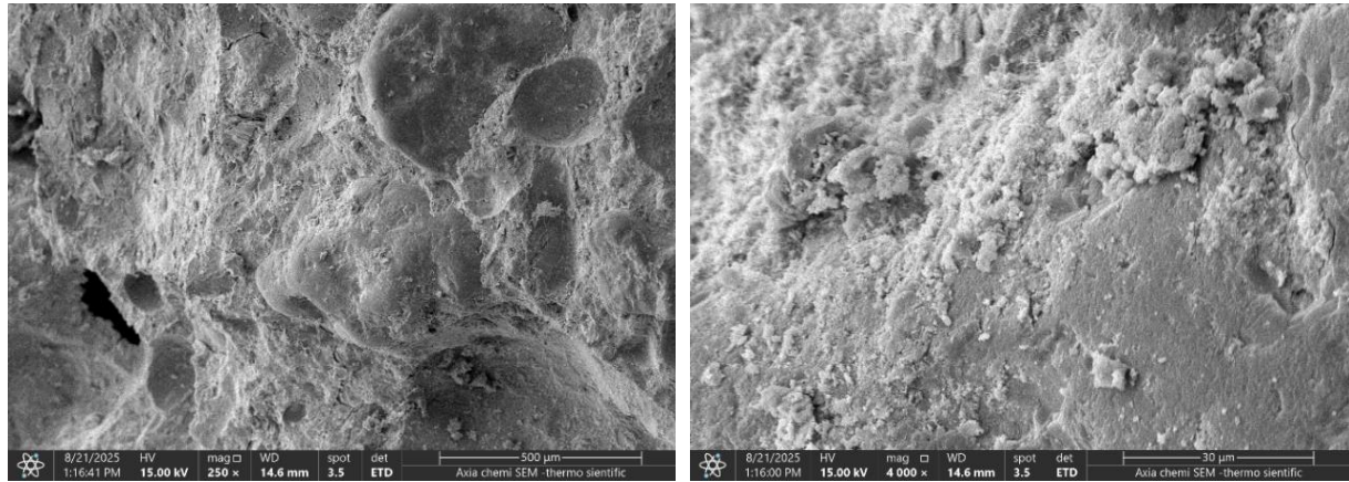
Fig. 15. The SEM of microstructure surface of control sample
